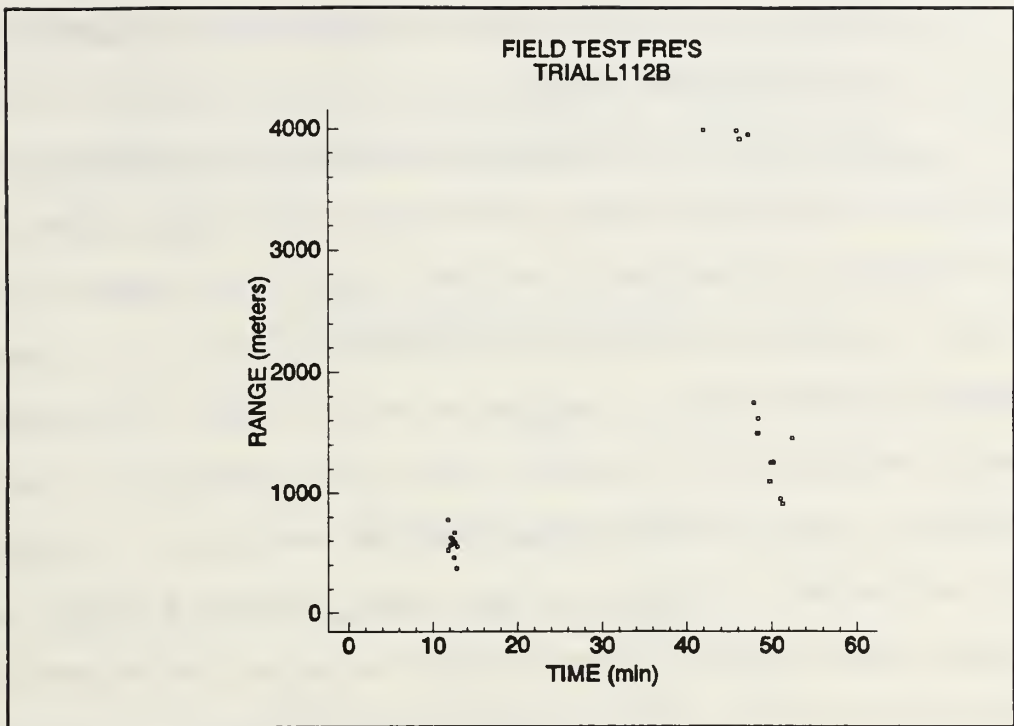
Figure 10 Range versus Time - Test
