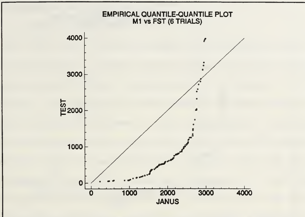
Figure 6 Q-Q Plot of pooled M1 vs FST FRE's (meters)
