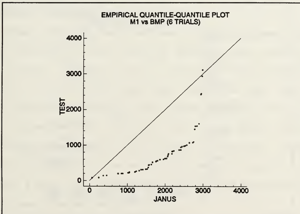
Figure 7 Q-Q Plot of pooled M1 vs BMP FRE's (meters)
