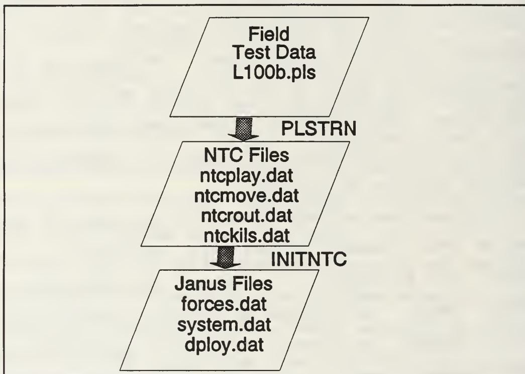
Figure 2 Conversion Process
