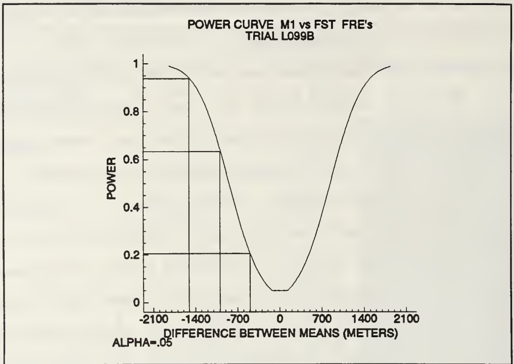
Figure 3 Power Curve (M1 vs FST)
