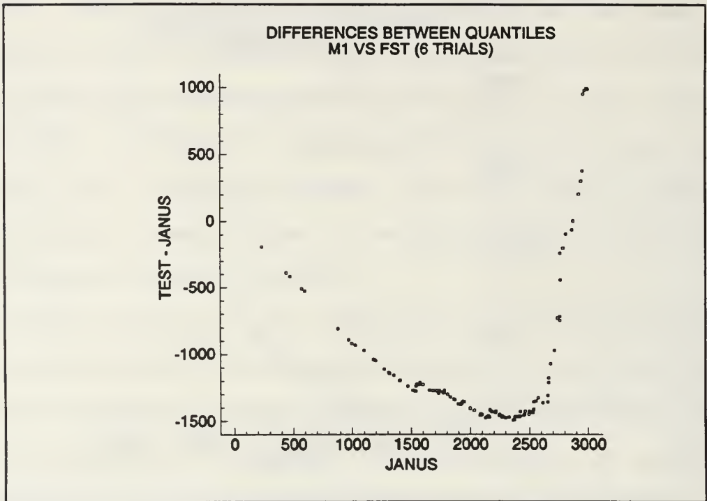
Figure 8 Differences Between Ranges (meters)
