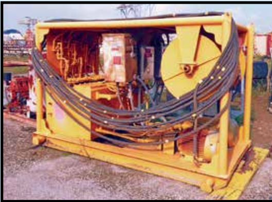
HYDRAULIC POWER UNIT FOR JACKING SYSTEMS
