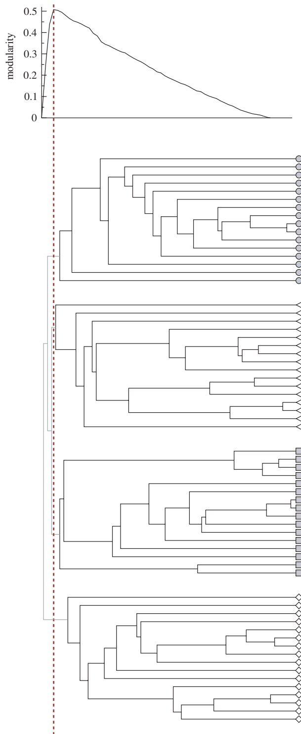
Fig. 7.3. Modularity Q (top panel) and dendrogram (bottom panel) obtained by the application of the GN algorithm to a computer generated modular random graph with 64 vertices and 256 edges. The random graph has been generated, as described in the text, by dividing the nodes into 4 groups of 16 nodes each (respectively empty circles, full circles, triangles and squares) and by considering z_{\text{in}} = 6 , z_{\text{out}} = 2 . The peak in the modularity (dotted line) corresponds to a perfect identification of the 4 communities.
