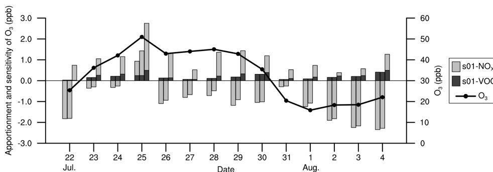
Figure 8. Sensitivities derived by BFM-20 (left) and BFM-100 (middle) and apportionments derived by ISAM (right) of daily ozone concentrations (shown by a line with markers) to the \text{NO}_x and VOC emissions of s01 for the 2 target weeks during the summer in ST.
