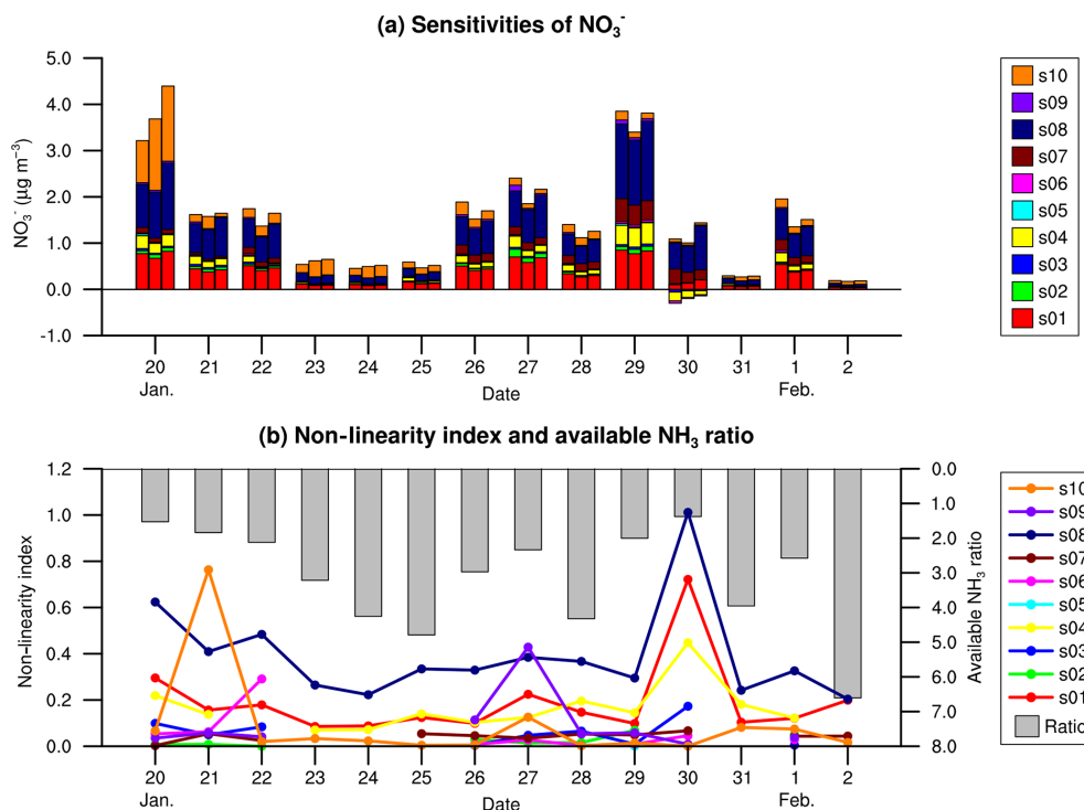
Figure 7. (a) Sensitivities of the daily \text{NO}_3^- concentrations to the source groups located within d02 (s01–s10) derived by BFM (left), HDDM-20 (middle), and HDDM-100 (right) and (b) daily non-linearity index and available \text{NH}_3 ratios for the 2 target weeks in winter in ST. Non-linearity indices for first-order sensitivity coefficients less than 0.001 \mu\text{g m}^{-3} are not shown as they are likely to be affected by numerical noise.
