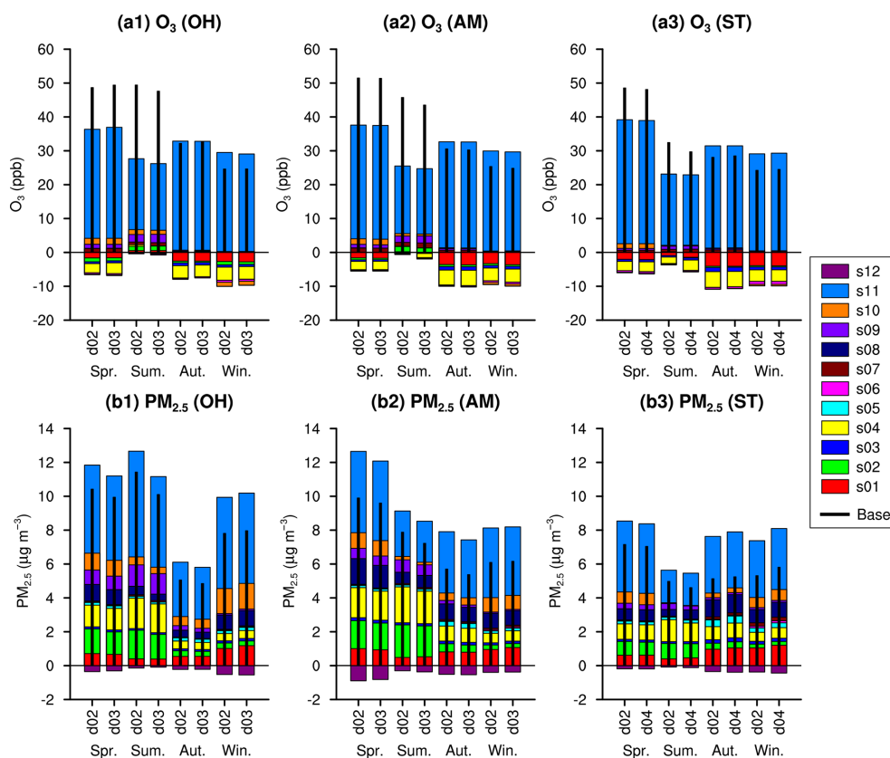
Figure 5. Sensitivities of the simulated ozone and \text{PM}_{2.5} concentrations to all source groups over OH, AM, and ST evaluated in d02, d03, and d04 for the 2 target weeks in the four seasons.
