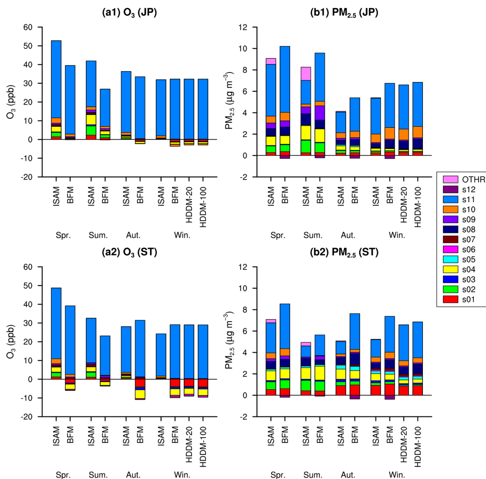
Figure 6. Apportionments derived by ISAM and sensitivities derived by BFM and HDDM of the simulated ozone and \text{PM}_{2.5} concentrations to all source groups in JP and ST for the 2 target weeks in the four seasons.
