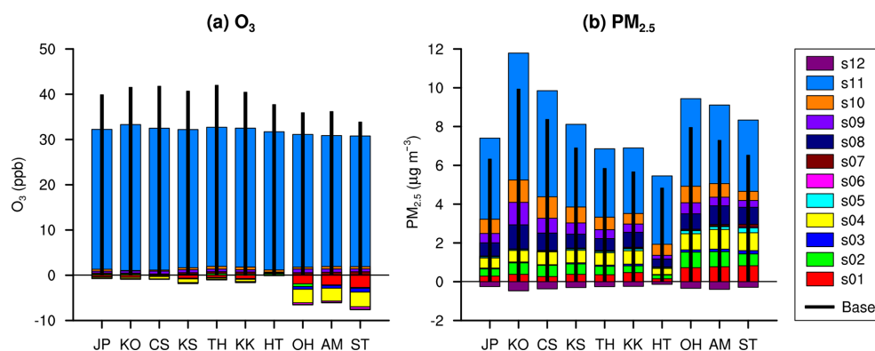
Figure 2. Source sensitivities of the annual mean ozone and PM 2.5 concentrations derived by BFM in the regions. Thick black lines represent the simulated concentrations.
