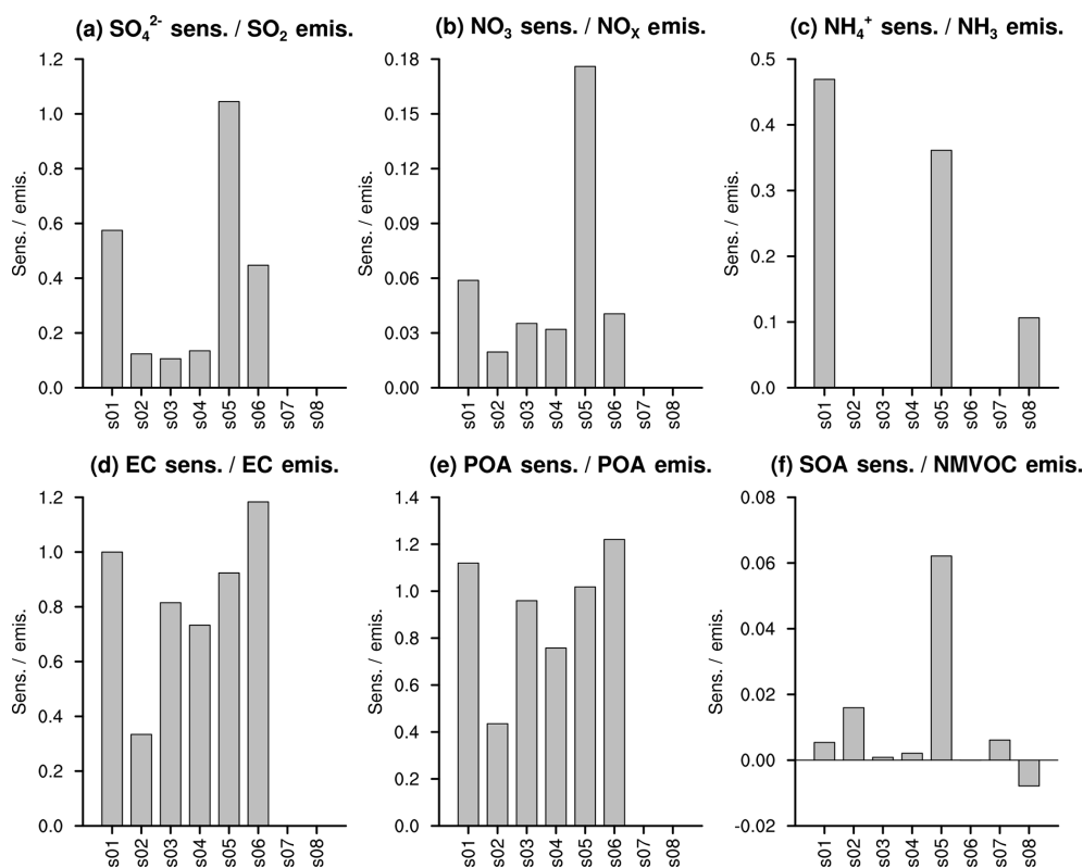
Figure 4. Sensitivities of the annual mean ambient concentrations of PM 2.5 components in d02 per total annual amount of corresponding precursor emissions from domestic anthropogenic sources (s01–s08) in all of Japan. All of them are normalized by the EC value for s01.
