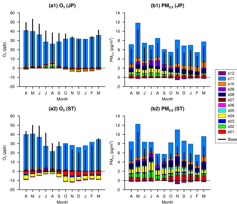
Figure 3. Source sensitivities of the monthly mean ozone and \text{PM}_{2.5} concentrations derived by BFM in all of Japan (JP) and ST. Thick black lines represent the simulated concentrations.
