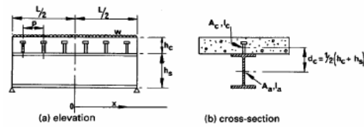
Fig. 2.15 Simply-supported composite beam.
