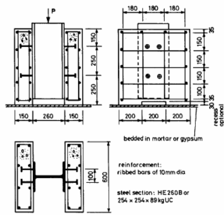
2.9 Standard push test.
