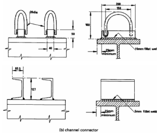
Fig. 2.7 Other types of shear connector.
