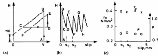
Fig. 2.23 Results of a slip-block test.
