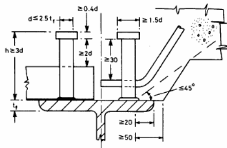
Fig. 3.24 Detailing rules for shear connection.
