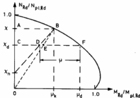
Fig. 5.13 Interaction curve for compression and uniaxial bending.
