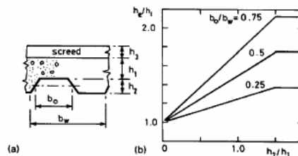
Fig. 3.7 Effective thickness of composite slab.
