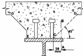
Fig. 2.13 Detailing rules for haunches.
