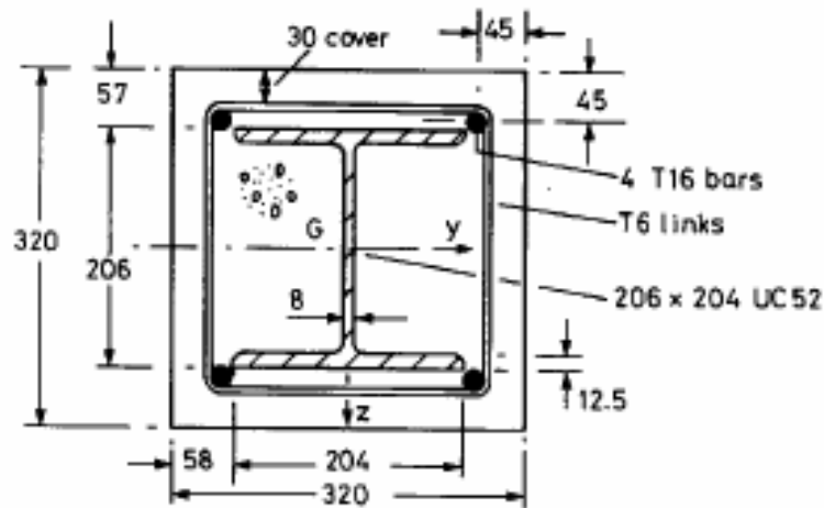
Fig. 5.15 Cross-section of external column.
