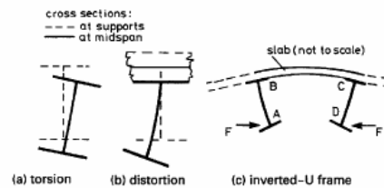
Fig. 4.3 Lateral buckling.
