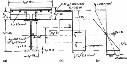
Fig. 4.1 Cross-section and stress distributions for composite beam in hogging bending.
