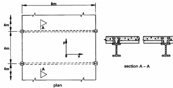
Fig. 3.1 Design example – structure for a typical floor.
