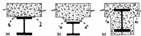
Fig. 2.1 Typical cross-sections of composite beams.
