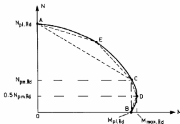
Fig. 5.14 Polygonal approximations to interaction curve.
