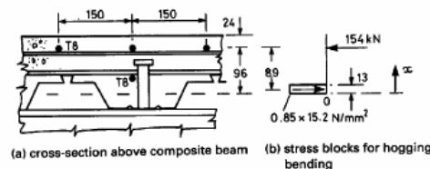
Fig. 3.12 Composite slab – design for fire.
