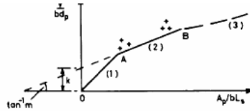
Fig. 2.21 Definition of m and k .
