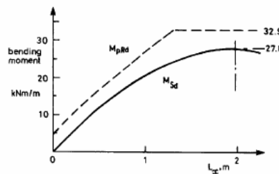
Fig. 3.11 Partial-interaction method, for longitudinal shear.
