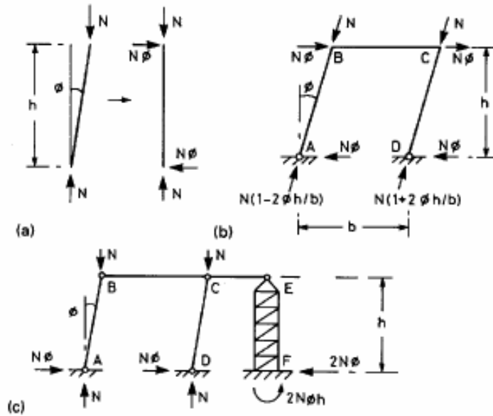
Fig. 5.6 Unbraced and braced frames.
