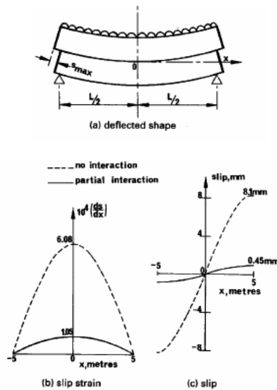
Fig2.3 Deflections, slip strain and slip
