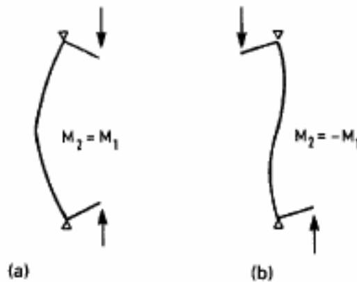
Fig. 5.12 Single-curvature and double-curvature bending.
