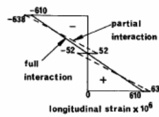
Fig. 2.17 Longitudinal strains at midspan.
