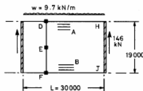
Fig. 5.8 Plan of typical floor slab.
