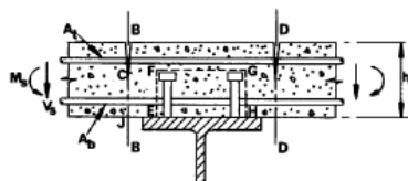
Fig. 3.20 Surfaces of potential failure in longitudinal shear.
