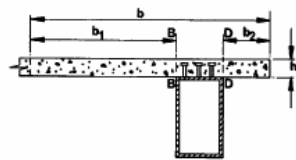
Fig. 3.21 T-beam with asymmetrical concrete flange.
