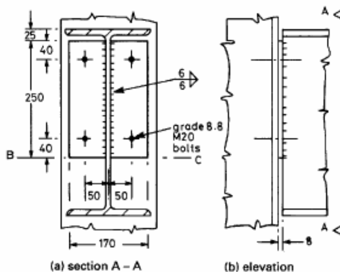
Fig. 5.17 Beam-to-column connection.
