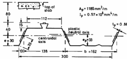
Fig. 3.9 Typical cross-section of CF 700.9 profiled steel sheeting.
