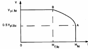
Fig. 4.2 Resistance to combined bending and vertical shear.
