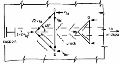
Fig. 3.22 Truss model for transverse reinforcement.
