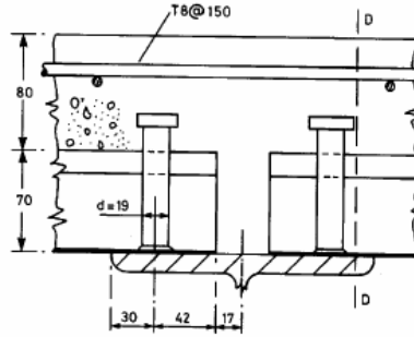
Fig. 3.30 Detail of shear connection.
