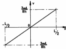
Fig.2.4 shear flow for 'triangular' spacing of connectors.
