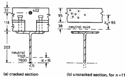
Fig. 4.14 Elastic properties of composite section.
