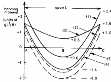
Fig. 4.9 Bending moment diagrams with redistribution
