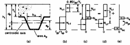
Fig. 3.2 Resistance of composite slab to sagging bending.
