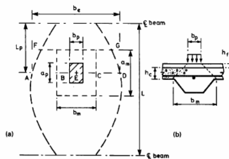
Fig. 3.6 Effective width of composite slab, for point load.
