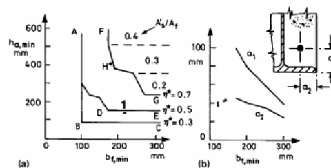
Fig. 3.28 Tabulated data for web-encased beams, class R60.
