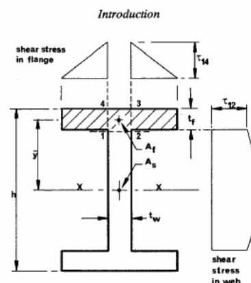
Fig. 1.2 Shear stresses in elastic I-section.
