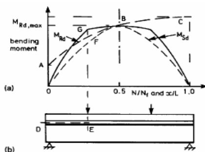
Fig. 3.17 Variation of bending resistance along a span.
