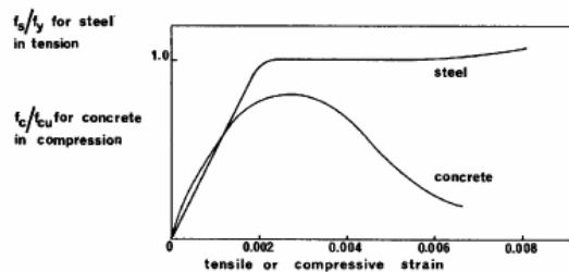
Fig. 1.1 Stress-strain curves for concrete and structural steel.
