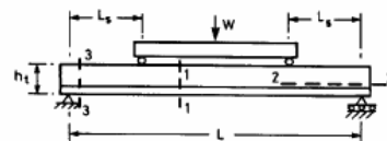
Fig. 2.19 Critical sections for a composite slab.
