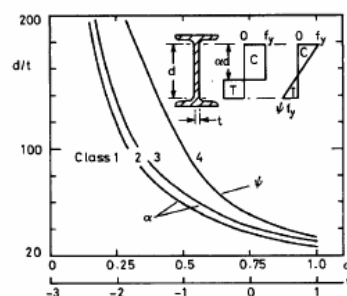
Fig. 3.14 Classification of webs, for f_y = 355 \text{ N/mm}^2 .
