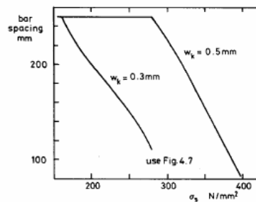
Fig. 4.8 Maximum bar spacing for high bond bars.
