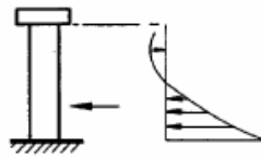
Fig 2.11 Bearing stress on the shank of a stud connector.
