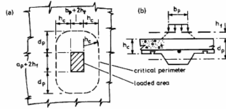
Fig. 3.5 Critical perimeter for punching shear.
