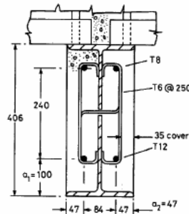
Fig. 3.31 Detail of concrete-encased web.
