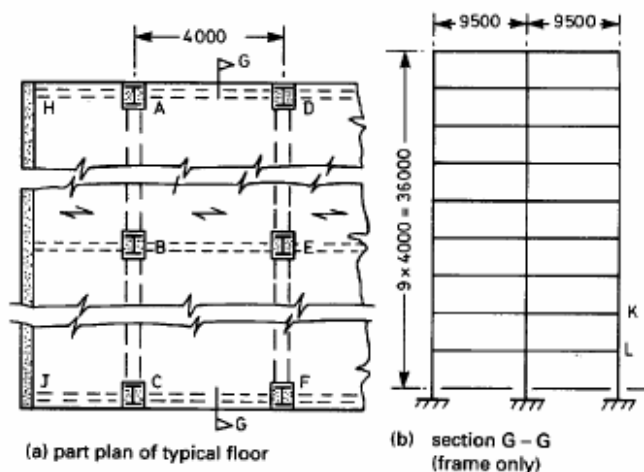
Fig. 5.1 A composite frame (simplified).
