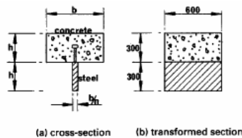
Fig .2.16 Transformed section of steel and concrete beam.
