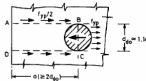
Fig. 3.23 Bearing resistance of profiled sheeting.
