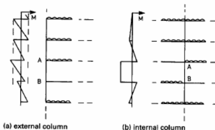
Fig. 5.7 Arrangements of imposed load, for column design.
