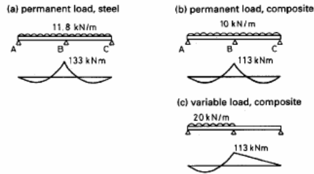
Fig. 4.13 Loading for deflection of span AB.
