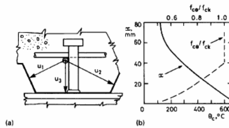
Fig. 3.8 Design data for temperatures in composite slab.
