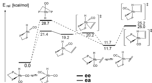
Fig. 13 Potential energy profile for the early catalytic steps (until migratory insertion) of the ethylene hydroformylation catalysed by [\text{HRh}(\text{CO})_2(\text{thioxantphos})] .
