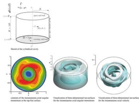
Figure 1. Use of CFD in engineering design. Simulation of an open transitional swirling (Bouffanaïs and Lo Jacono, 2009) flow.
