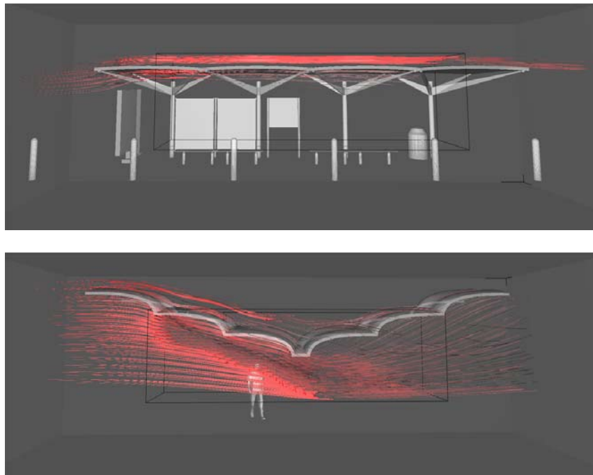
Figure 7 Visualization of a CFD analysis result using custom developed toolkit: Visualization of wind flow above 1.3 m/s coming into the space of interest. Top: Existing bus stop design commonly encountered in Singapore. Bottom: Proposed bus stop design.
