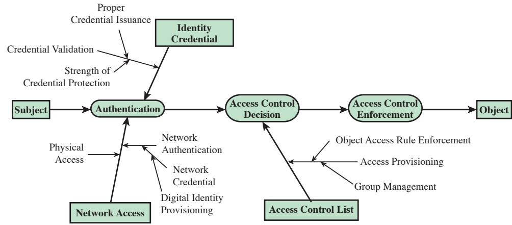
(a) ACL Trust Chain
