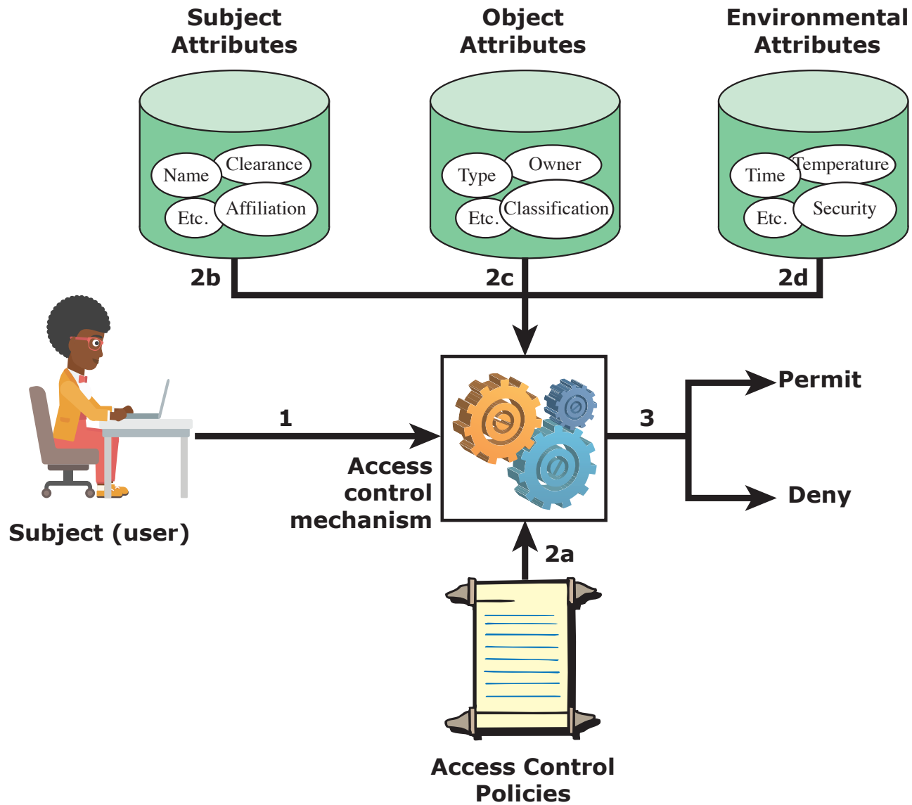
Figure 4.10 ABAC Scenario
