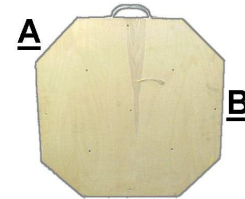
Treated Birch Plywood Pad 23½ x 23½ x 3" A = 7½, B = 13"
