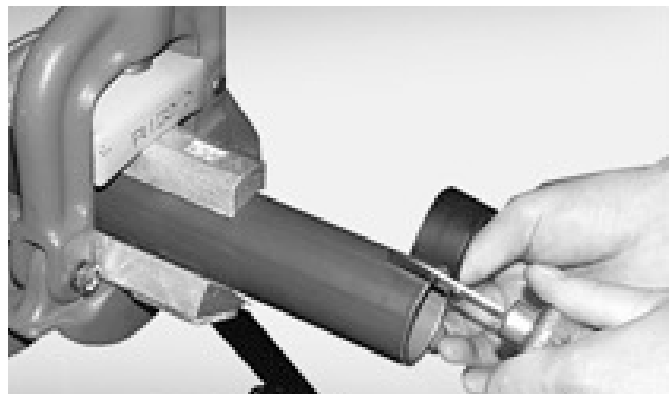
Figure 17: Before threading PVC-coated conduit, make a series of cuts along the axis of the conduit to break-up threading chip.
