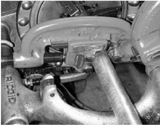
Figure 5: Lower the roll cutter to the desired length. Tighten the handle about one quarterturn per each revolution and repeat until conduit is cut through.
