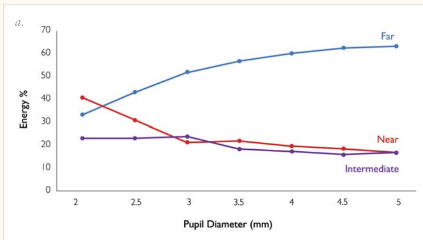
Figure 1. a. The light distribution of the Lucidis IOL – available in two sizes (10.8 mm and 12.4 mm) with a power range of +5.0 D to 30.0 D, in steps of 0.5 D; b. The refractive and aspheric optical elements with the innovative closed-loop haptic design to give an optimal centration; c. The pseudo non-diffracting beam approach providing a constant resolution and light intensity on the retina.
