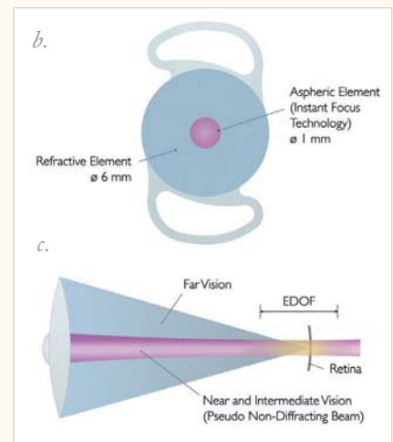
Figure 1. a. The light distribution of the Lucidis IOL – available in two sizes (10.8 mm and 12.4 mm) with a power range of +5.0 D to 30.0 D, in steps of 0.5 D; b. The refractive and aspheric optical elements with the innovative closed-loop haptic design to give an optimal centration; c. The pseudo non-diffracting beam approach providing a constant resolution and light intensity on the retina.
