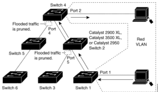
Figure 8-2 Optimized Flooded Traffic with VTP Pruning
