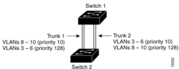
Figure 8-4 Load Sharing by Using STP Port Priorities
