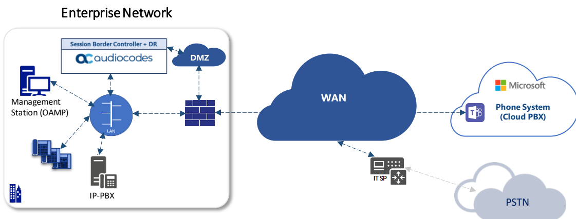
Figure 2-2: Connection Topology with SIP Trunk on the WAN
