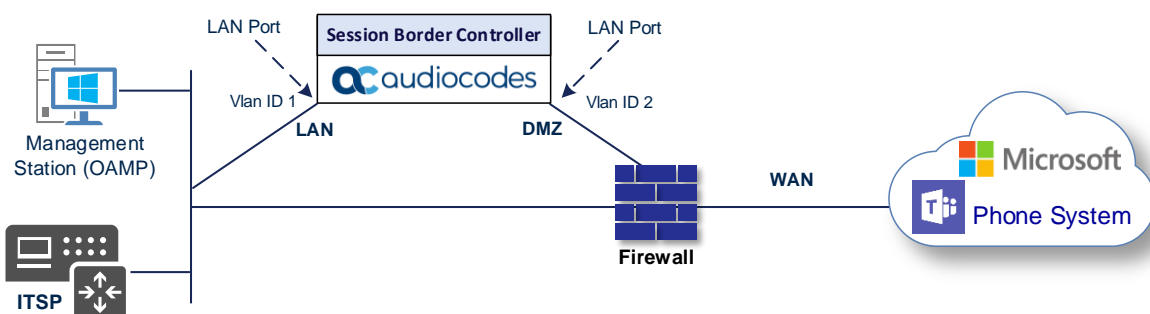
Figure 4-3: Network Interfaces in the Topology with SIP Trunk on the WAN
