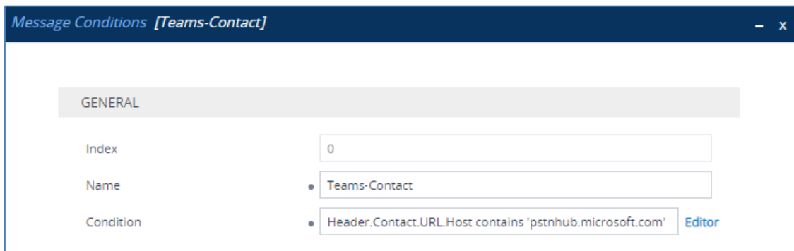
Figure 4-22: Configuring Condition Table
