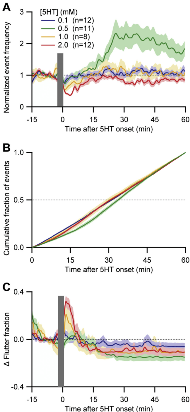
Fig. 6. Effect of 5HT on EPG activity in A. ceylanicum L4s. A. Dose-response relationship of normalized event frequency (pumps + flutters) versus 5HT concentration. At t = 0 min, perfusate was switched (grey bar) from control medium (RPMI-c with 20% CS) to the same medium with different concentrations of 5HT (see key). Lines and shading show mean \pm S.E.M.; n (number of worms) shown in key. Dotted line marks normalized frequency of 1.0. B. Cumulative fraction of events for 60 min after switching to 5HT-containing perfusate. CF_{50} values (dotted line) did not differ significantly between groups except for the 0.5 mM 5HT group, which differed from all other groups ( P < 0.04 ; 2-tailed Wilcoxon Mann-Whitney U test). C. Change ( \Delta ) in 'flutter fraction,' (the proportion of total EPG events that were flutters); baseline flutter fraction was between 0.05 and 0.2 in all groups (not shown). Dotted line marks zero change in flutter fraction. Same data set in A–C. All recordings at 34–36 °C.
