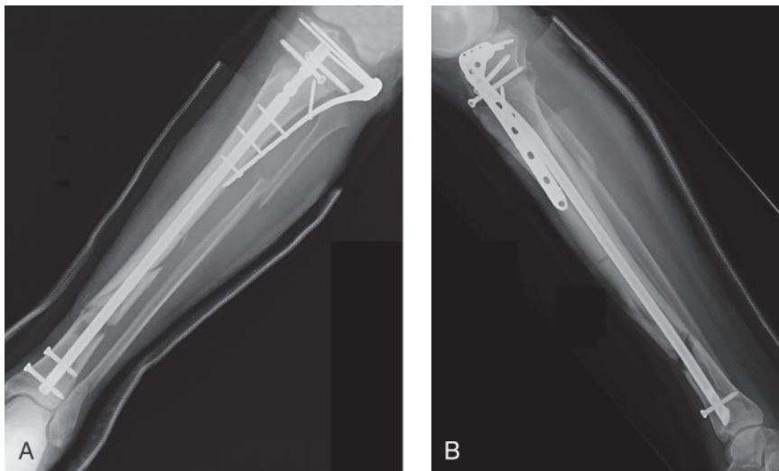
Figure 1 AP (A) and lateral (B) radiographs demonstrating bicortical reduction plating. Careful plate application allows for secure fixation of an unstable proximal tibia fracture before nailing.
