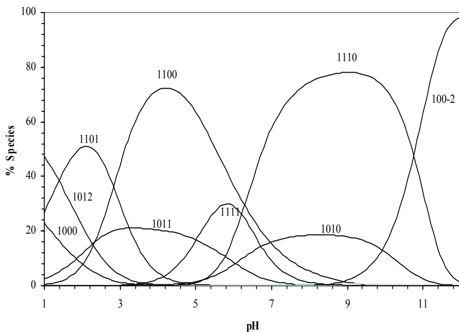
Fig. 5. Concentration distribution of various species as a function of pH in the Pd(Pic)-CBDCA-IMP system at concentrations of 1.25 \times 10^{-3} mol-dm ^{-3} for Pd(Pic) ^{2+} ; CBDCA and IMP, I = 0.1 mol-dm ^{-3} (NaNO _3 ) and T = 25 \pm 0.1 °C).
