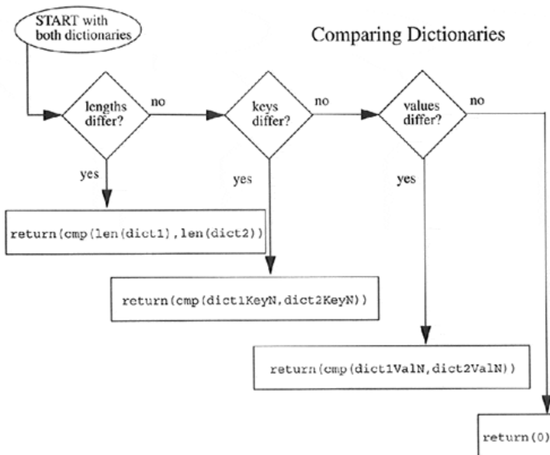
Figure 7-1. How Dictionaries are Compared
