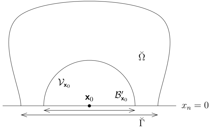
Figure 2.1: Local configurations (\check{\Omega}, \check{\Gamma}) and (\check{\mathcal{V}}_{\mathbf{x}_0}, \check{\mathcal{B}}'_{\mathbf{x}_0}) .
