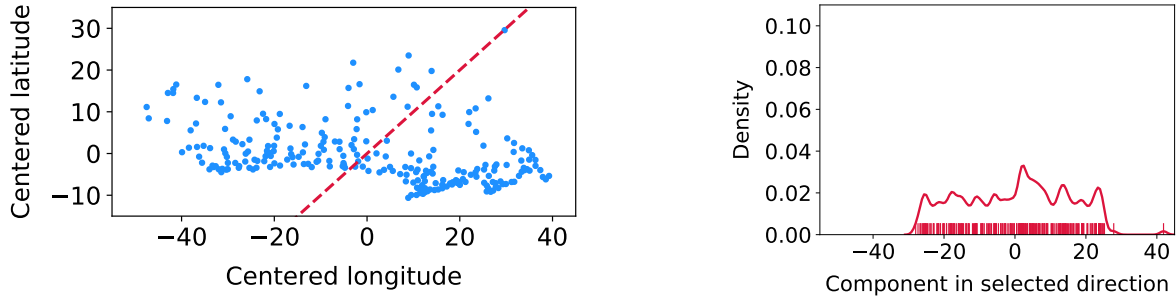
Figure 2: Sample variance in southwest-northeast direction. The left scatterplot shows the centered data from Figure 1, and a fixed direction of the two-dimensional space represented by a line going through the origin from southwest to northeast. The right plot shows the components of each data point in the direction of the line and a kernel density estimate. The sample standard deviation of the components is 15.1.
