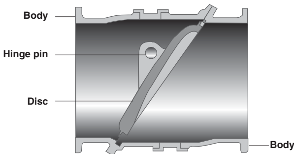
TILTING DISC
