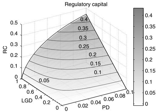
(a) RC: \varrho = 20\% , M=1 (3D)
