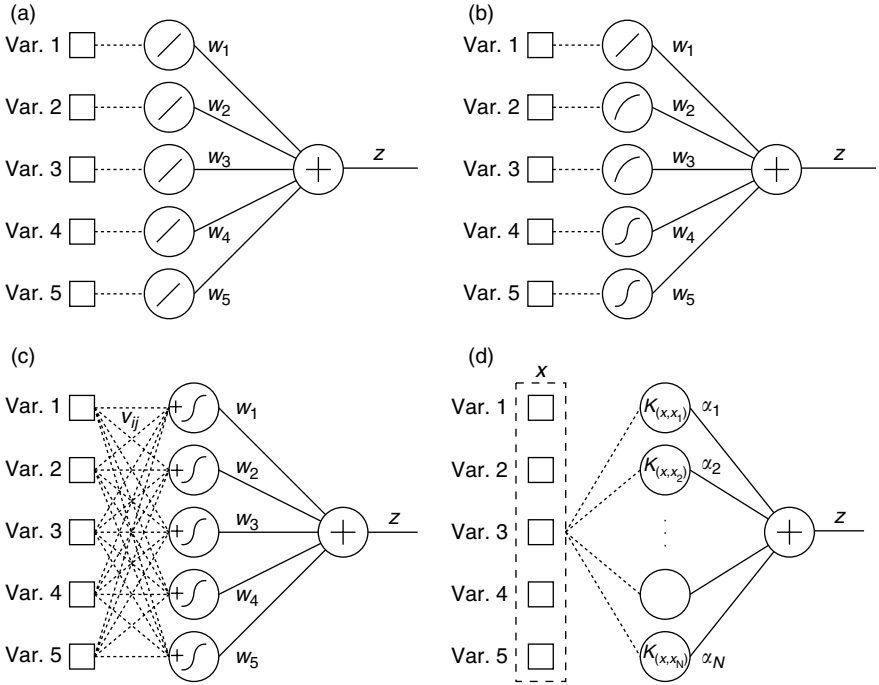
Fig. 4.5 Model architectures to compute the z -score from the input variables x_1, \dots, x_5 (var. 1, \dots , var. 5). The linear (a), intrinsically linear (b) and MLP model (c) are parametric models with increasing complexity and learning capability. The SVM or kernel-based model (d) is a non-parametric model where the learning capacity depends, a.o., on the choice of the kernel function K .
