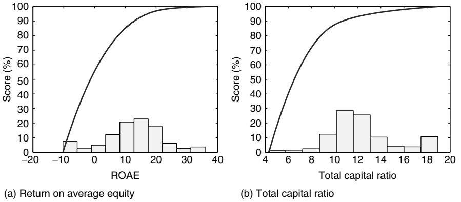
Fig. 4.6 Visualization of the identified univariate non-linear transformations for the total capital ratio and the return on average equity in a model for rating banks. The Basel Capital Accord requires a minimum total capital ratio of 8%. Values below 8% are increasingly penalized. For values higher than 10%, a saturation effect occurs. The same holds for the ROAE. Values above 10% are not rewarded further. Negative returns, i.e. losses, are increasingly penalized. More details can be found in [488]. The ratio distribution is indicated by the histograms.
