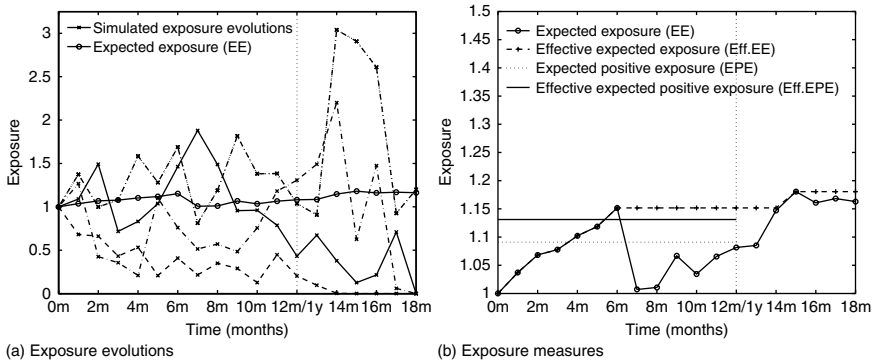
Fig. 4.18 Counterpart credit risk exposure evolutions are depicted in the left pane for the case of two call options with maturity 6 and 18 months. Observe that the exposure levels may fluctuate significantly due to market price fluctuations. The level of these fluctuations depends on the diversification of the contracts in the netting set. For a current exposure (CE) of €1, the exposure measures expected exposure (EE), effective expected exposure (Eff. EE), expected positive exposure (EPE) and effective expected positive exposure (Eff. EPE) are reported in the right pane.
