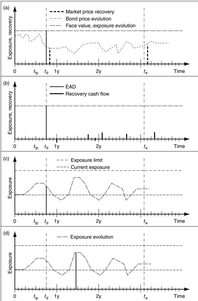
Fig. 4.14 Timeline of a distressed firm: last payment date ( t_{ip} ), default date t_d and emergence from default or settlement ( t_e ). The bankruptcy procedure may follow shortly after the default date t_d . The default definition impacts the LGD measurement and the EAD definition. Panels c and d depict the EAD definition, respectively, as the exposure at default and maximum exposure during default. In panels (a) and (b) the bond LGD is measured via the (discounted) bond market price recovery shortly after default or after emergence or settlement. The LGD can also be obtained from workout recovery cash flows (panel b).
