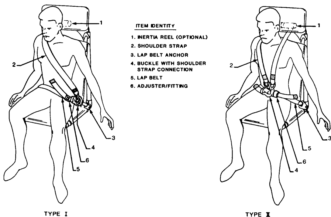
FIGURE 17. Troop Seat Restraint Configurations
