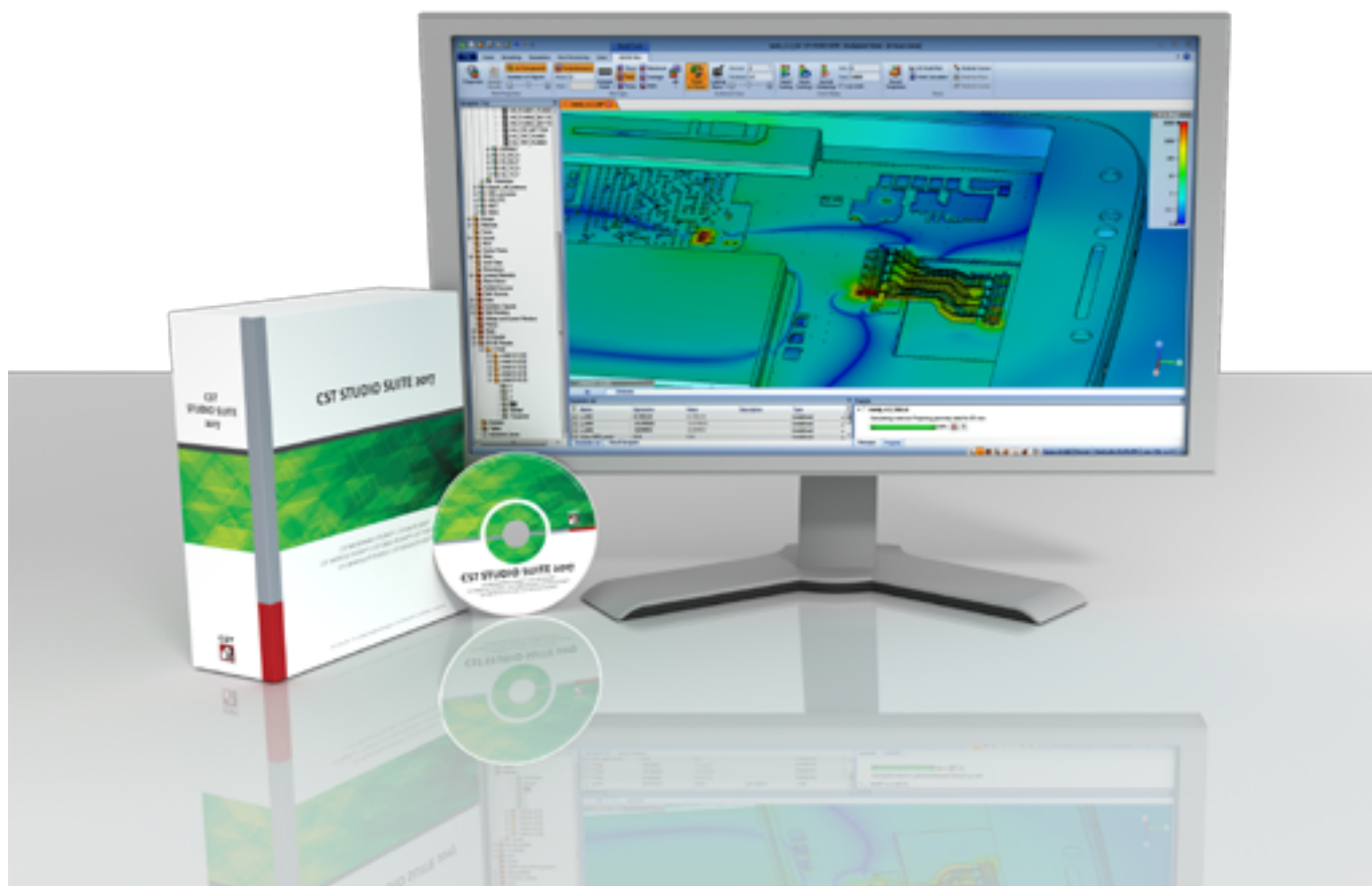
The CST STUDIO SUITE graphical user interface, showing E-fields inside a mobile phone. Simulation allows a detailed analysis of the entire phone, including antenna performance, specific absorption rate (SAR), electromagnetic compatibility (EMC) and signal integrity (SI).
