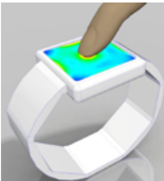
Screen stress: Abaqus/Standard.
