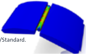
Signal Integrity: CST Time Domain Solver.
