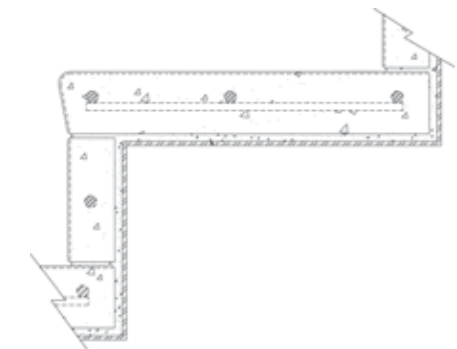
C40 SEPARATE TREAD & RISER
