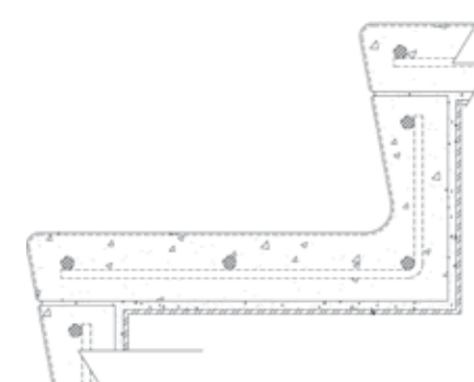
C36 REVERSE TREAD & RISER
