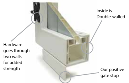
| INSIDE OF PATENTED GATE FRAME |
