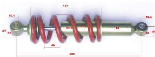
*PEUGEOT XP6 520510
