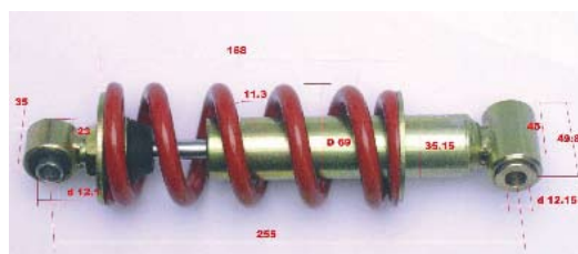
*YAMAHA TZR 50 520513 < 2004
