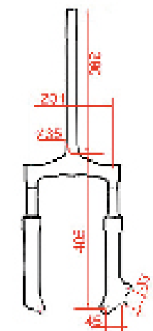
*STALKER 290140
