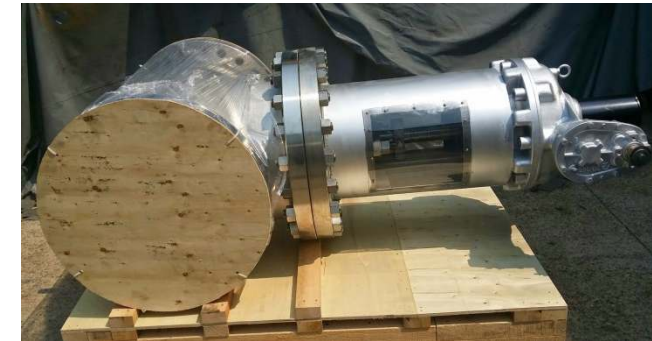
GLOBE VALVE APPLICATION : O2 30K 450A / OIL FREE
