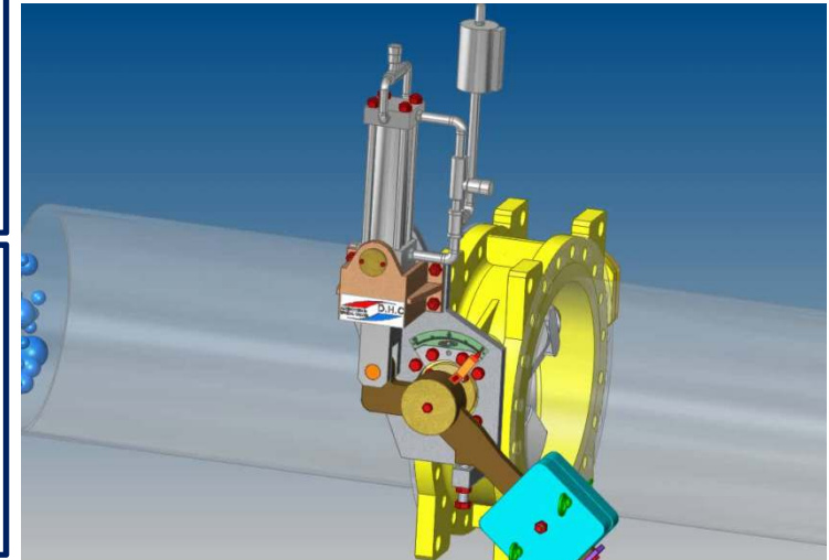
Operation of NSCV
