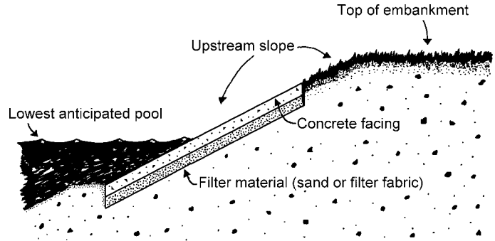
Figure 4 - Concrete facing
