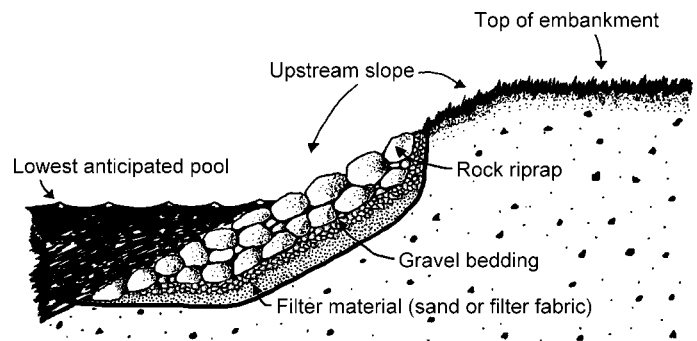
Figure 2 - Rock Riprap
