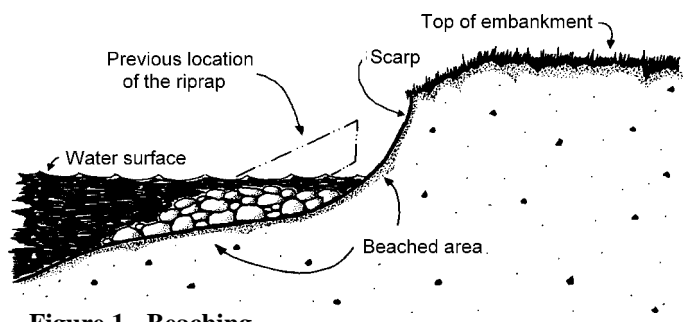
Figure 1 - Beaching
