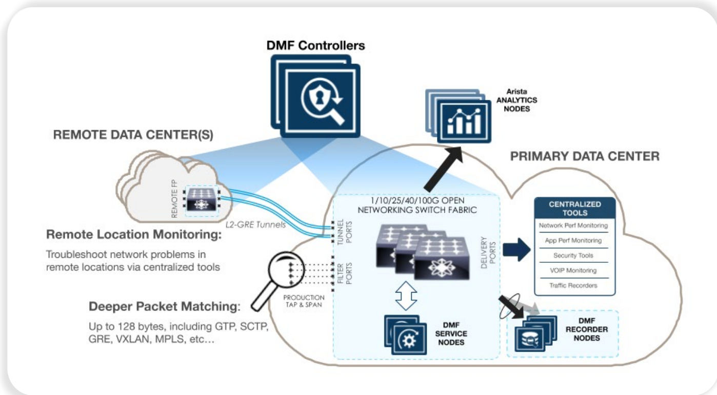
Figure 3: DANZ Monitoring Fabric - Monitor Every Location with Centralized Tools and Management
