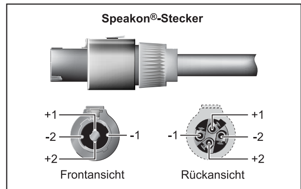
Abb. 4.1: Speakon®-Anschlüsse
