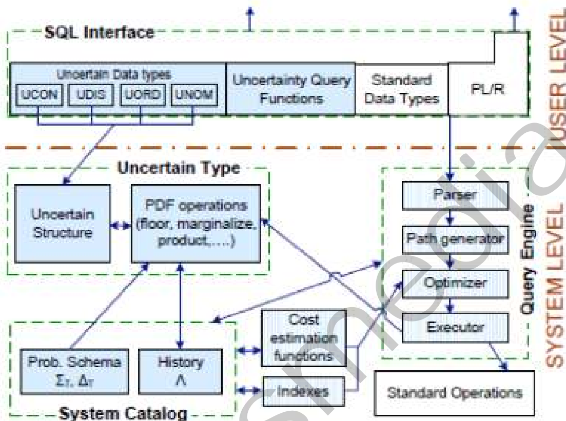
Figure 1: Orion 2.0 Architecture
