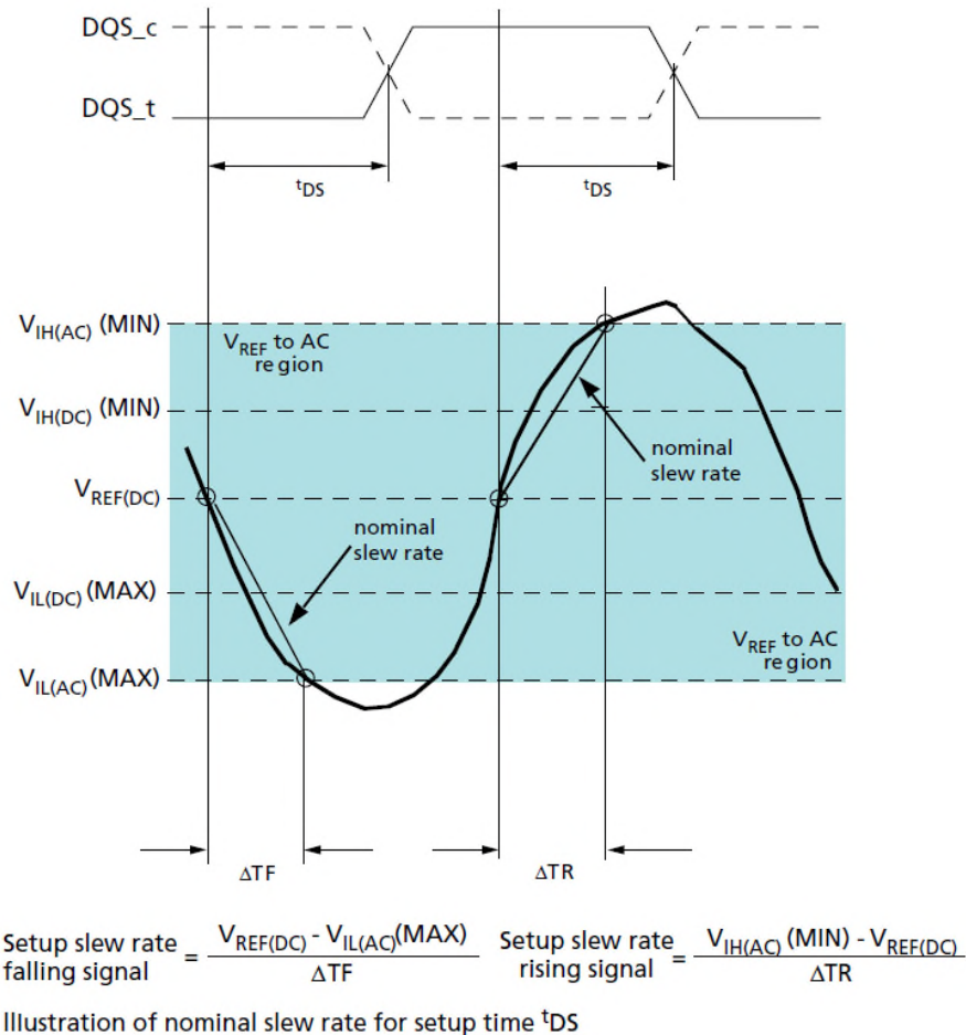
Figure 9: Nominal Slew Rate for Data Setup Time (t t DS), NV-DDR2/NV-DDR3 only
