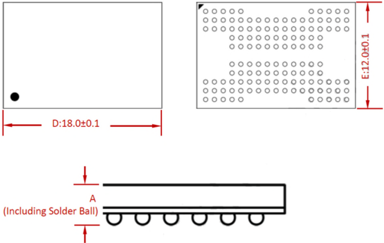
Figure 2: 132-Ball LPGA - 12mm x 18mm
