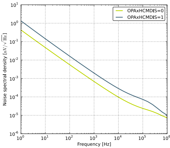
Figure 3.25. OPAMP Voltage Noise Spectral Density (Non-Unity Gain)
