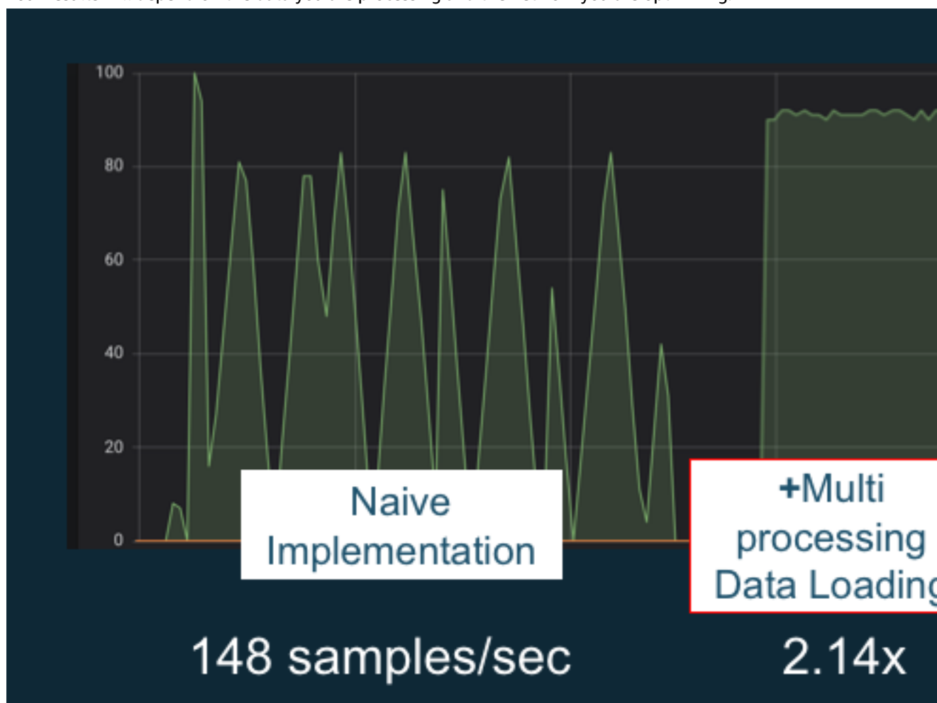
Example GPU performance optimizations. Chart source: Performance Tricks with MXNet Gluon
