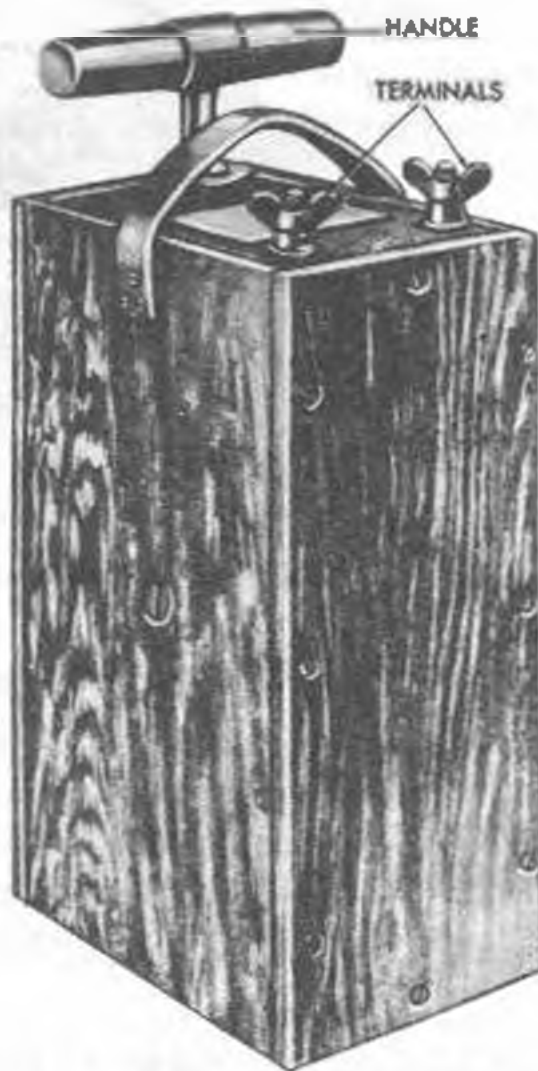
B—THIRTY-CAP BLASTING MACHINE
