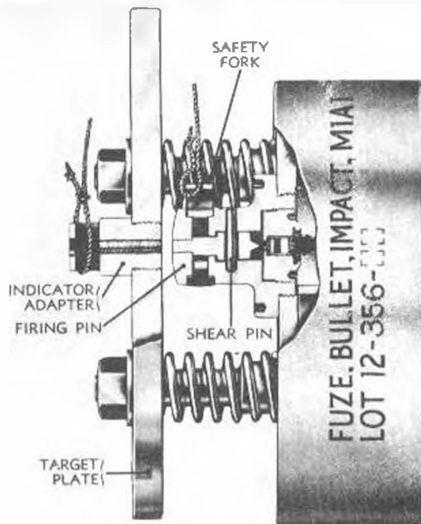
Figure 75. Fuze, bullet impact, M1A1—Cutaway and rear view.
