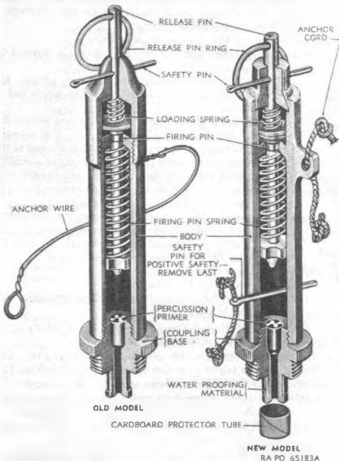
Figure 35. Firing device, pull type, M1—sectioned.
