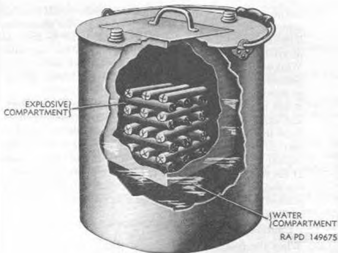
Figure 4. Dynamite-thawing kettle.
