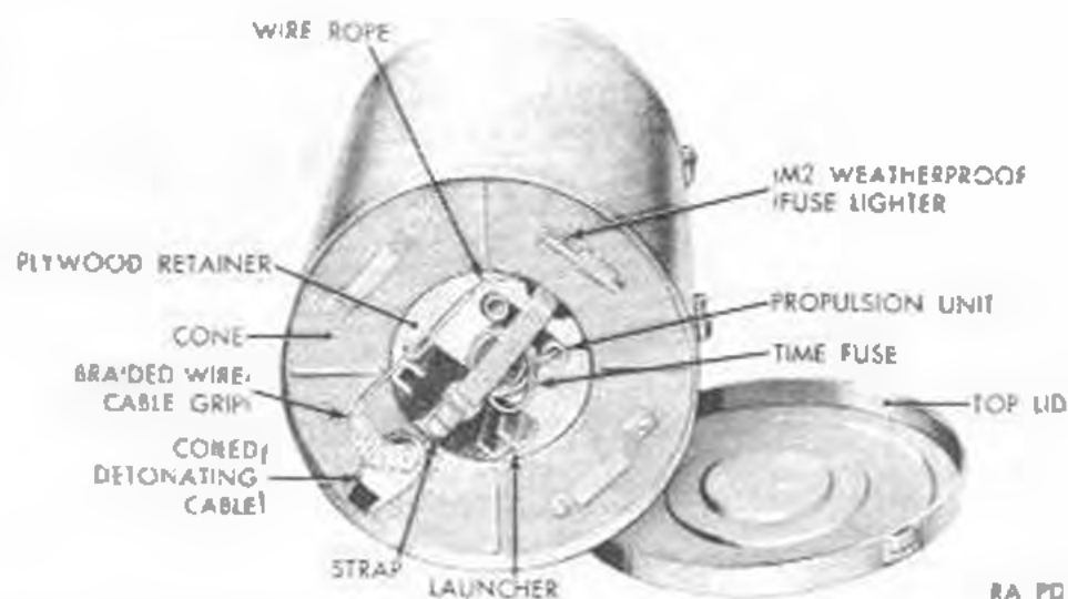
Figure 63. Cable, detonating, mine-clearing, antipersonnel, M1—top lid of case removed.
