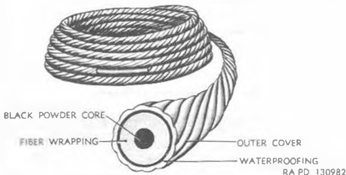
Figure 22. Fuse, blasting, time.
