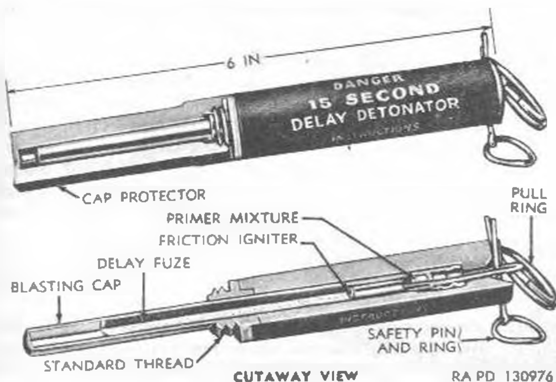
Figure 18. Detonator, 15-second delay, M1.
