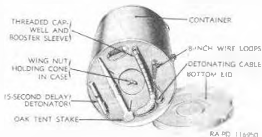
Figure 64. Cable, detonating, mine-clearing, antipersonnel, M1—bottom lid of case removed.
