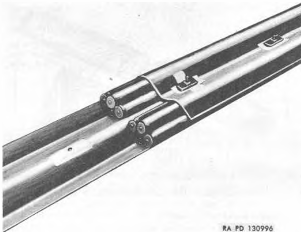
Figure 80. Demolition snake M3 loaded with bangalore torpedoes.
