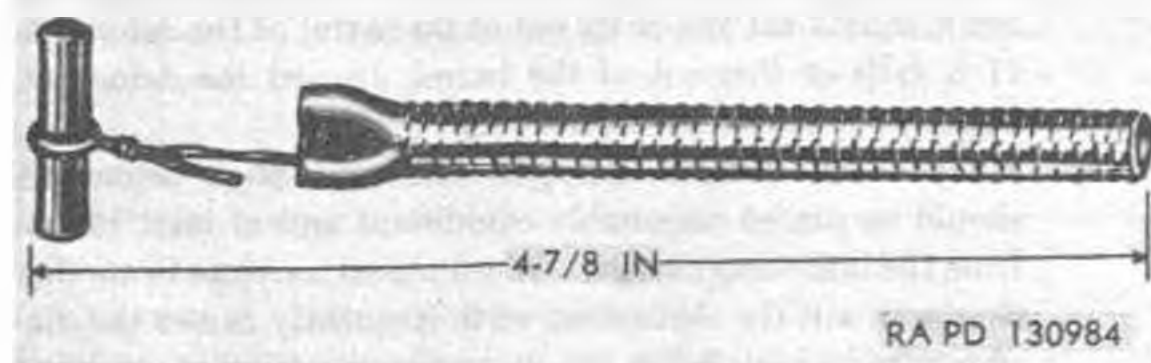
Figure 20. Lighter, fuse, friction-type, M1.
