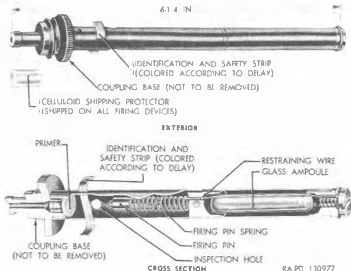
Figure 27. Firing device, delay type, M1.
