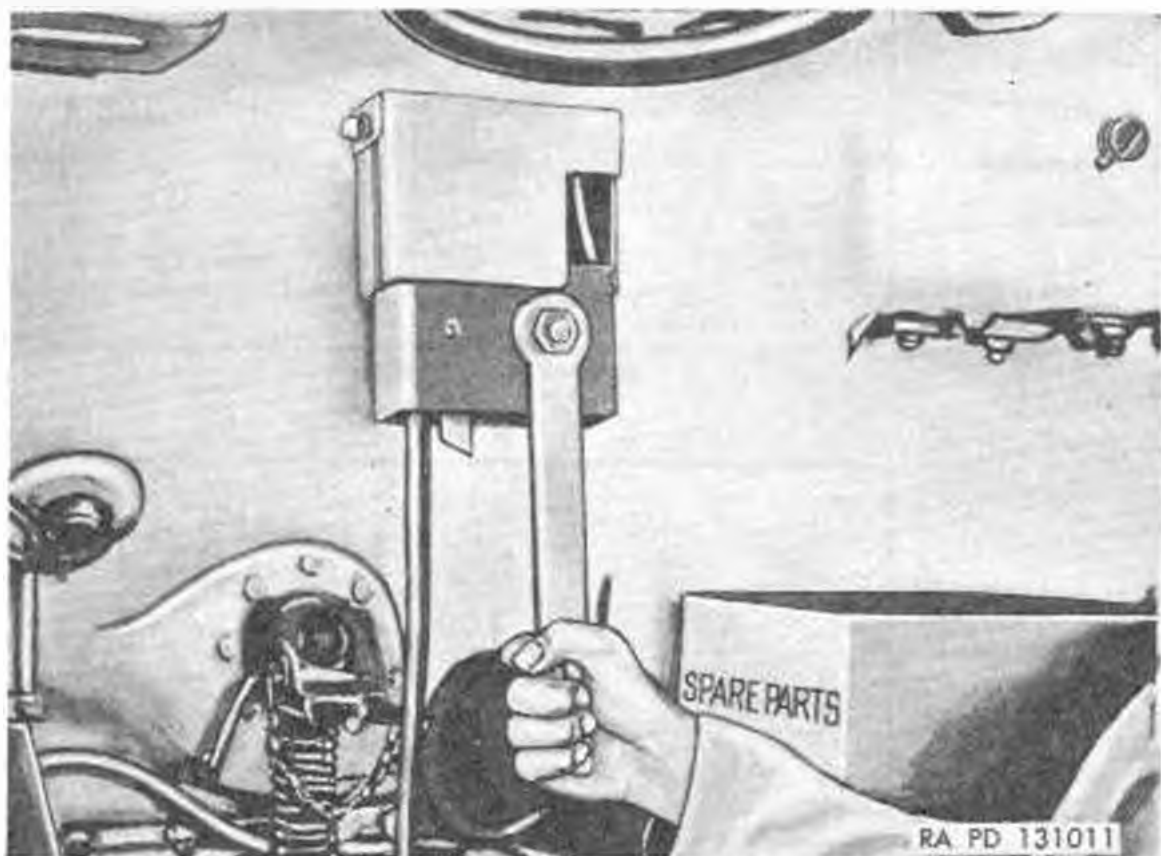
Figure 91. Medium tank bow gunner raising towing assembly with wrench issued with demolition snake M3.
