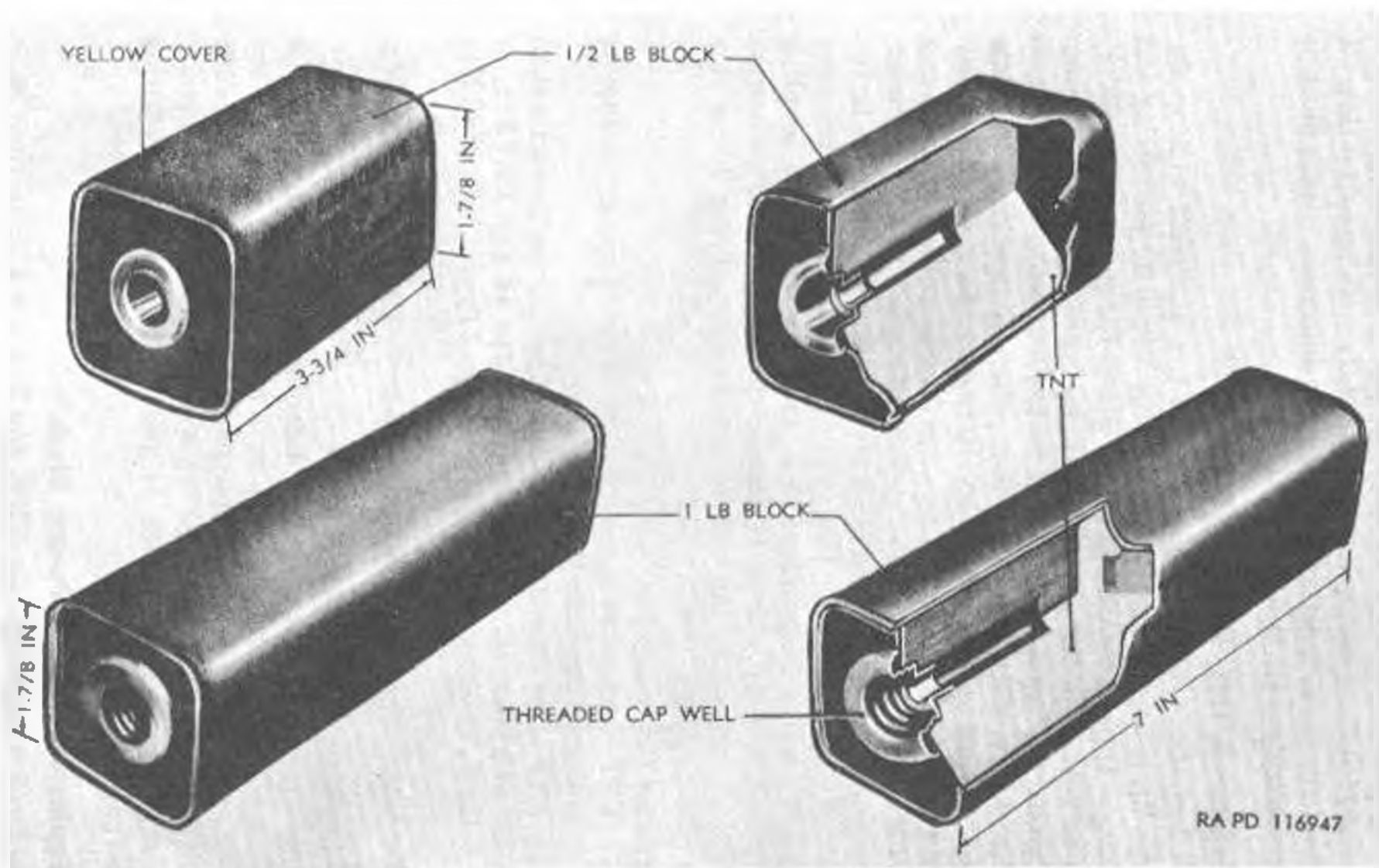
Figure 8. Explosive, TNT, 1/2 pound block, and explosive, TNT, 1 pound block.
