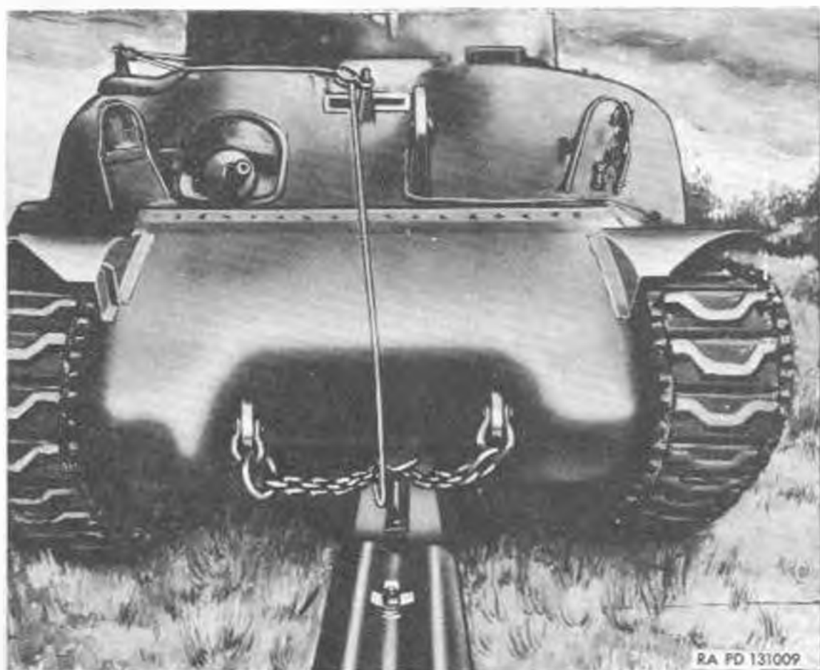
Figure R9. Pushing assembly, demolition snake M3.
