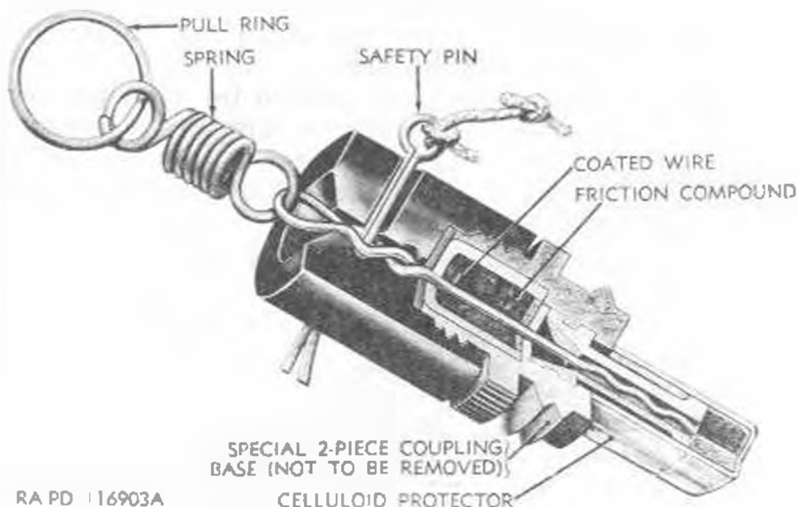
Figure 32. Firing device, pull friction type, M2—sectioned.
