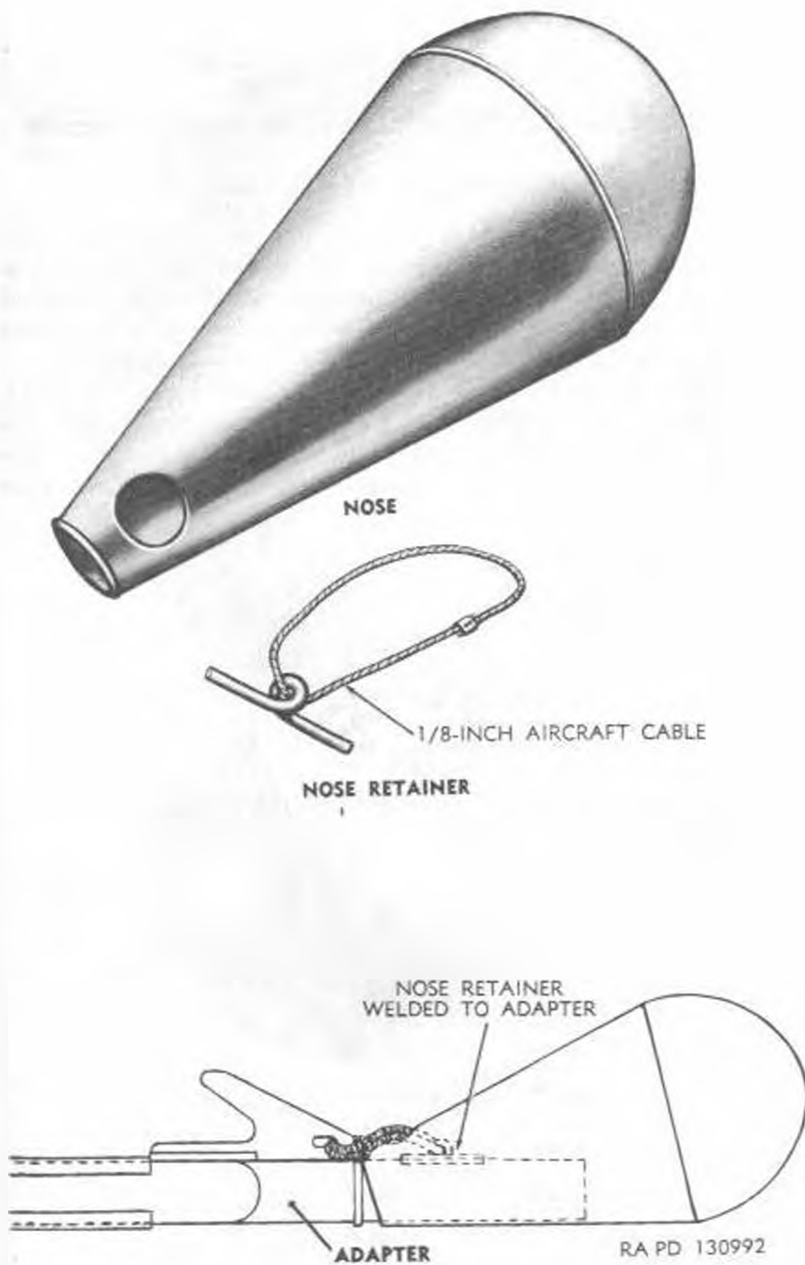
Figure 72. Nose and retainer, demolition snake M3.
