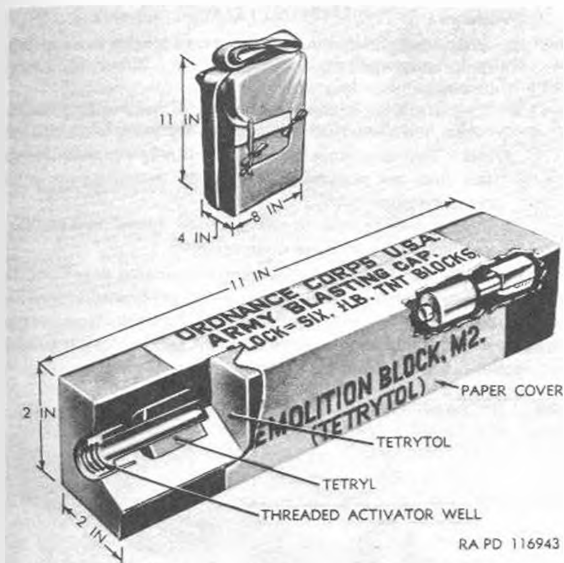
Figure 6. Block, demolition, M2—enlarged sectioned view and carrying haversack for eight blocks.
