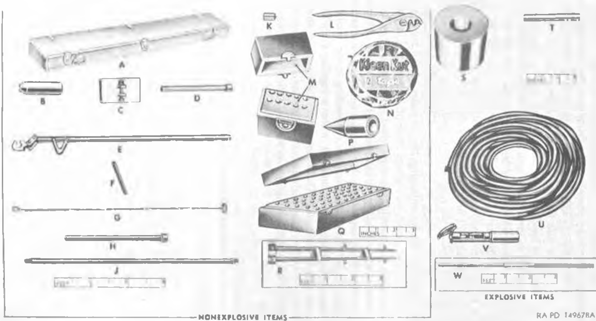
Figure 51. Rod, earth, blast-driven, set No. 1.
