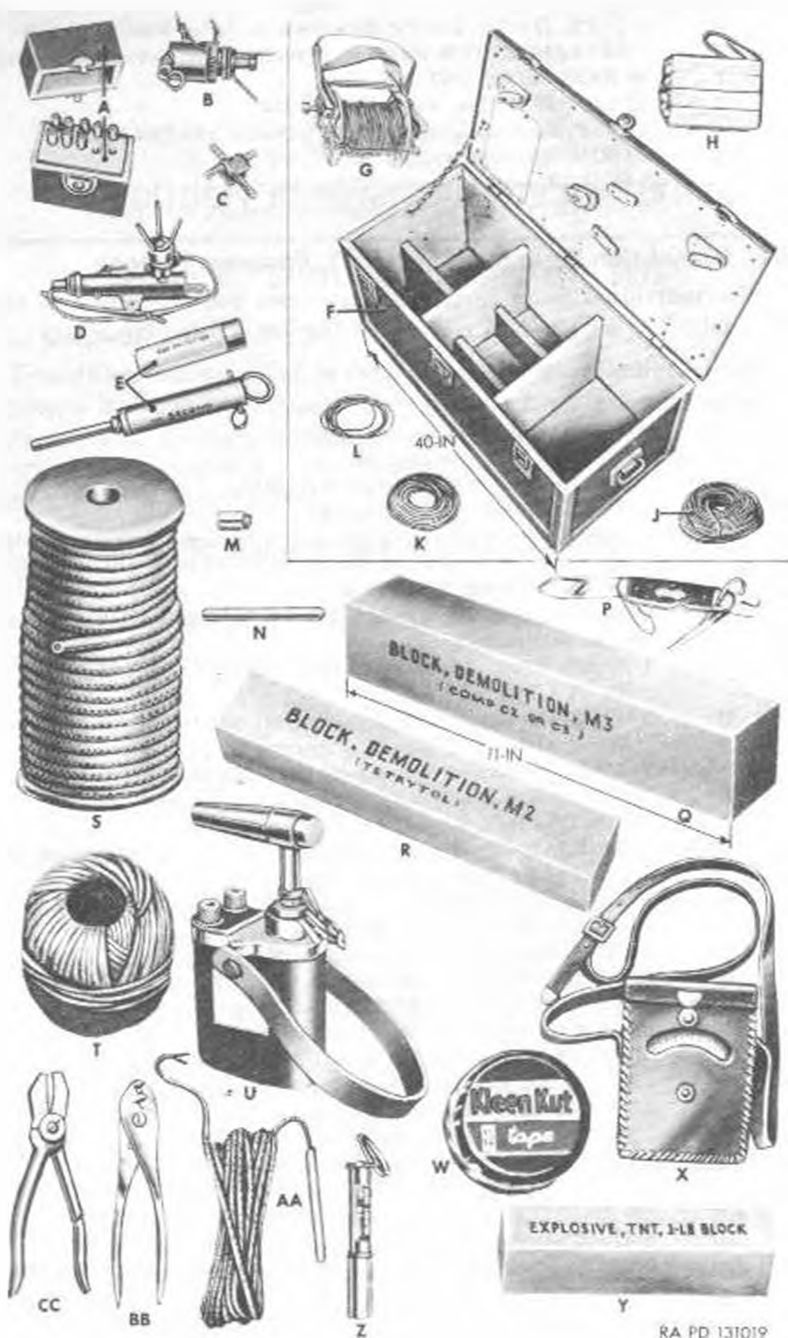
Figure 17. Demolition equipment set No. 1, Engineer Squad.
