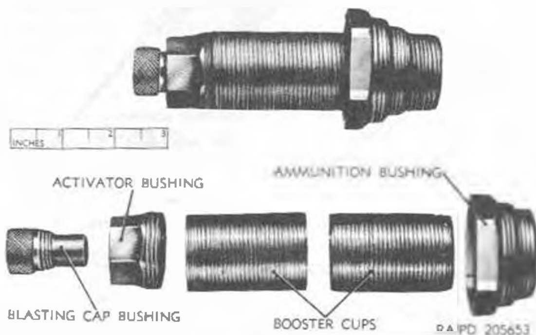
Figure 41. Destructor, High-explosive, universal, M10.
