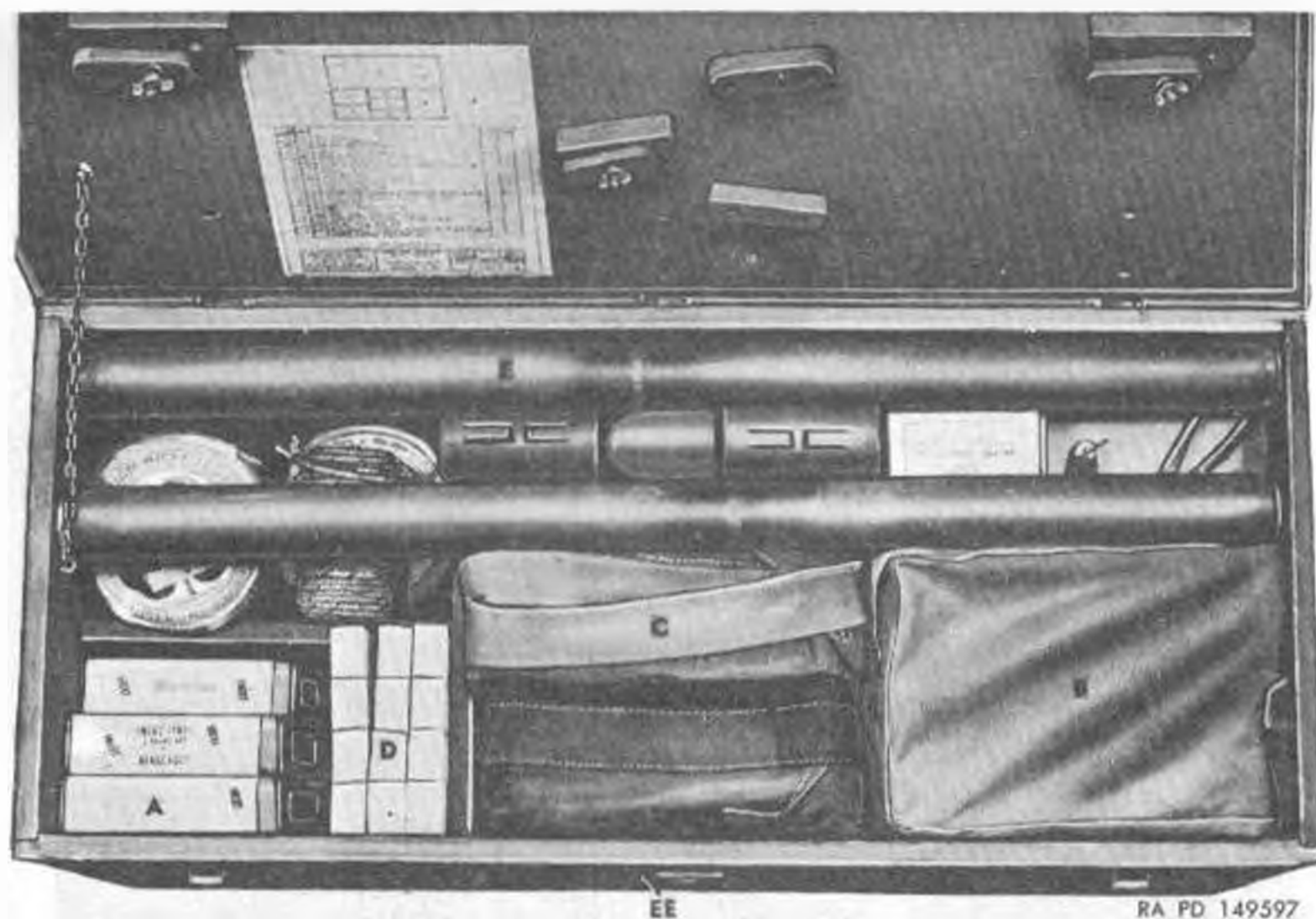
Figure 55. Demolition training kit T38—packing plan, top layer.
