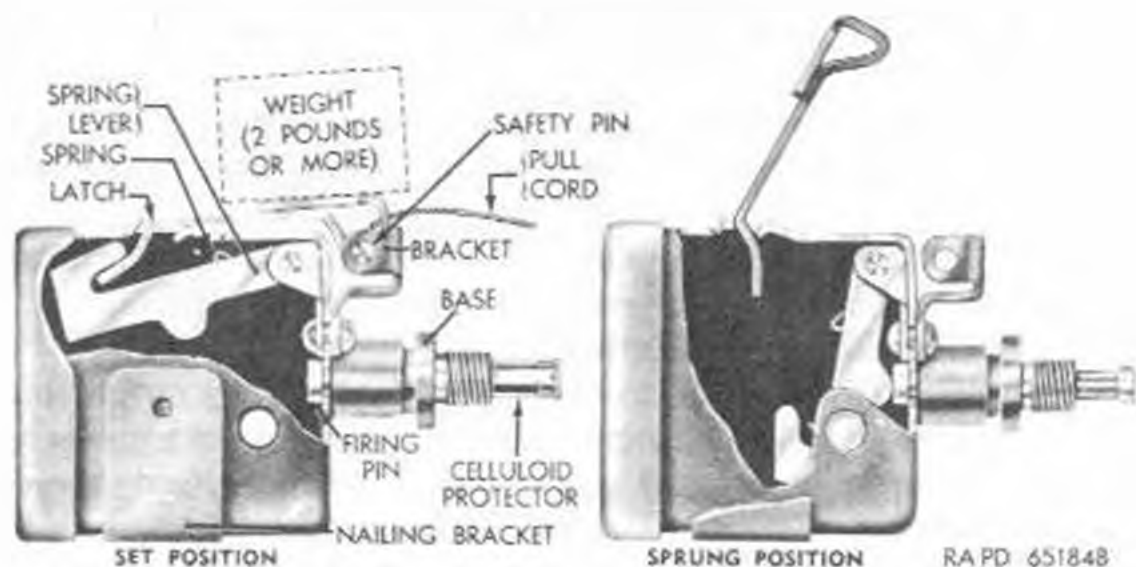
Figure 36. Firing device, release type, M1.
