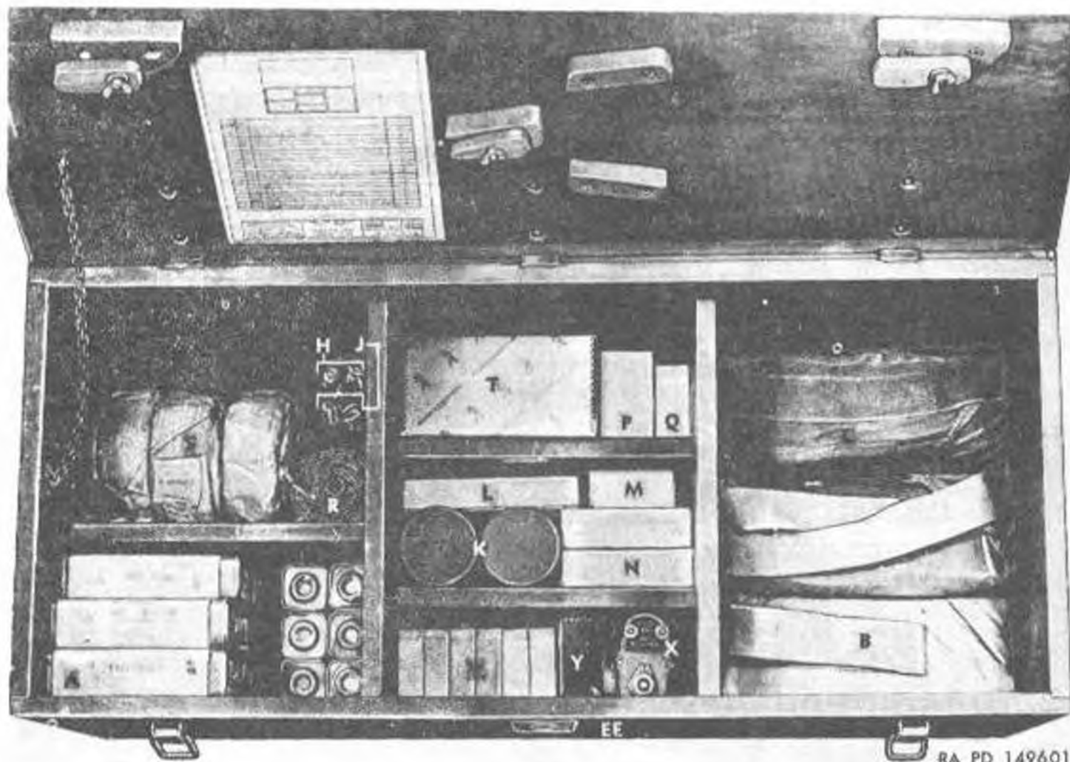
Figure 59. Demolition training kit T39 parking plan, top layer.
