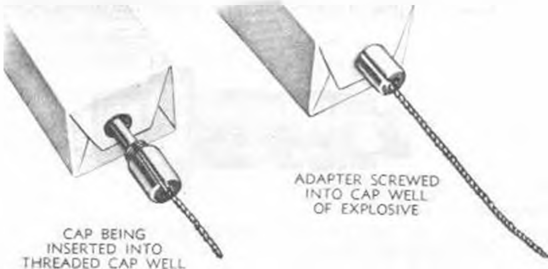
A—PRIMING ADAPTER USED WITH ELECTRIC BLASTING CAP
