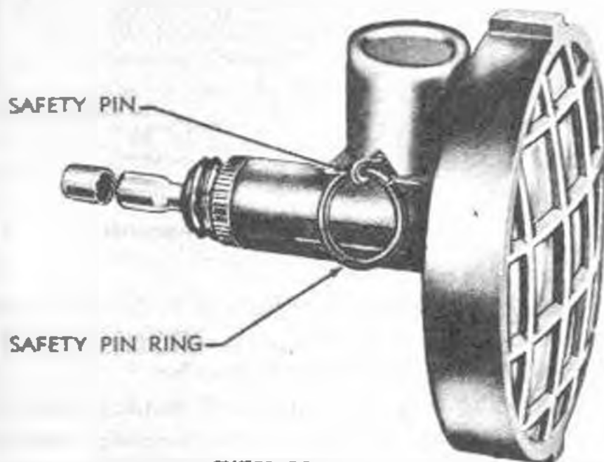
EXTERIOR— ASSEMBLED FOR INSTALLATION
