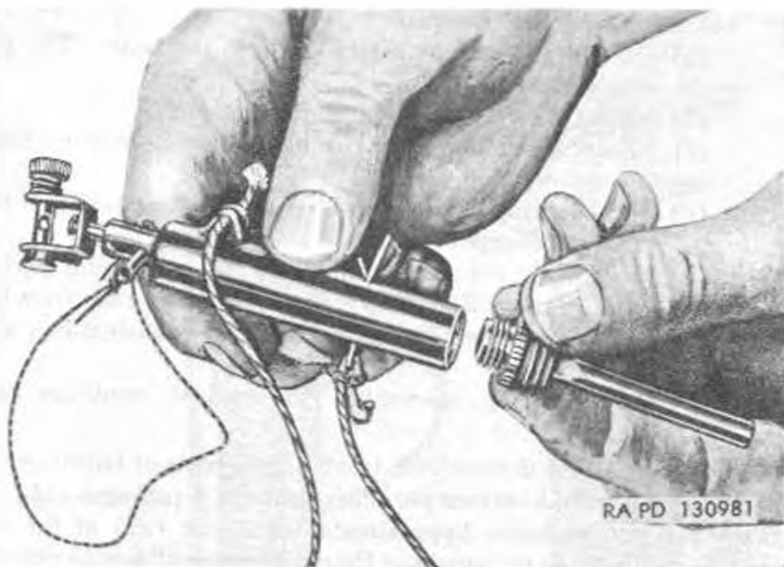
Figure 34. Assembling pull-release type firing mechanism to primed coupling base with crimped-on blasting cap.
