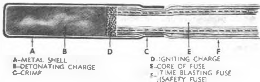
Figure 38. Caps—blasting.
