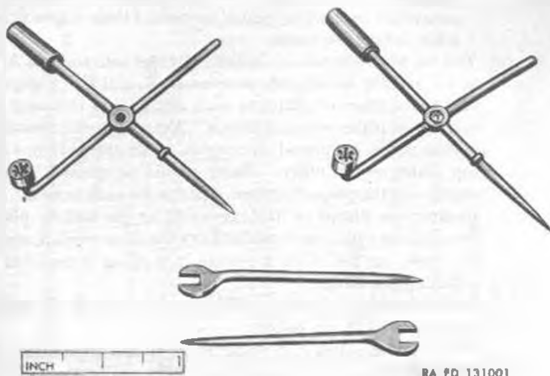
Figure 84. Assembly wrenches, demolition snake MS.
