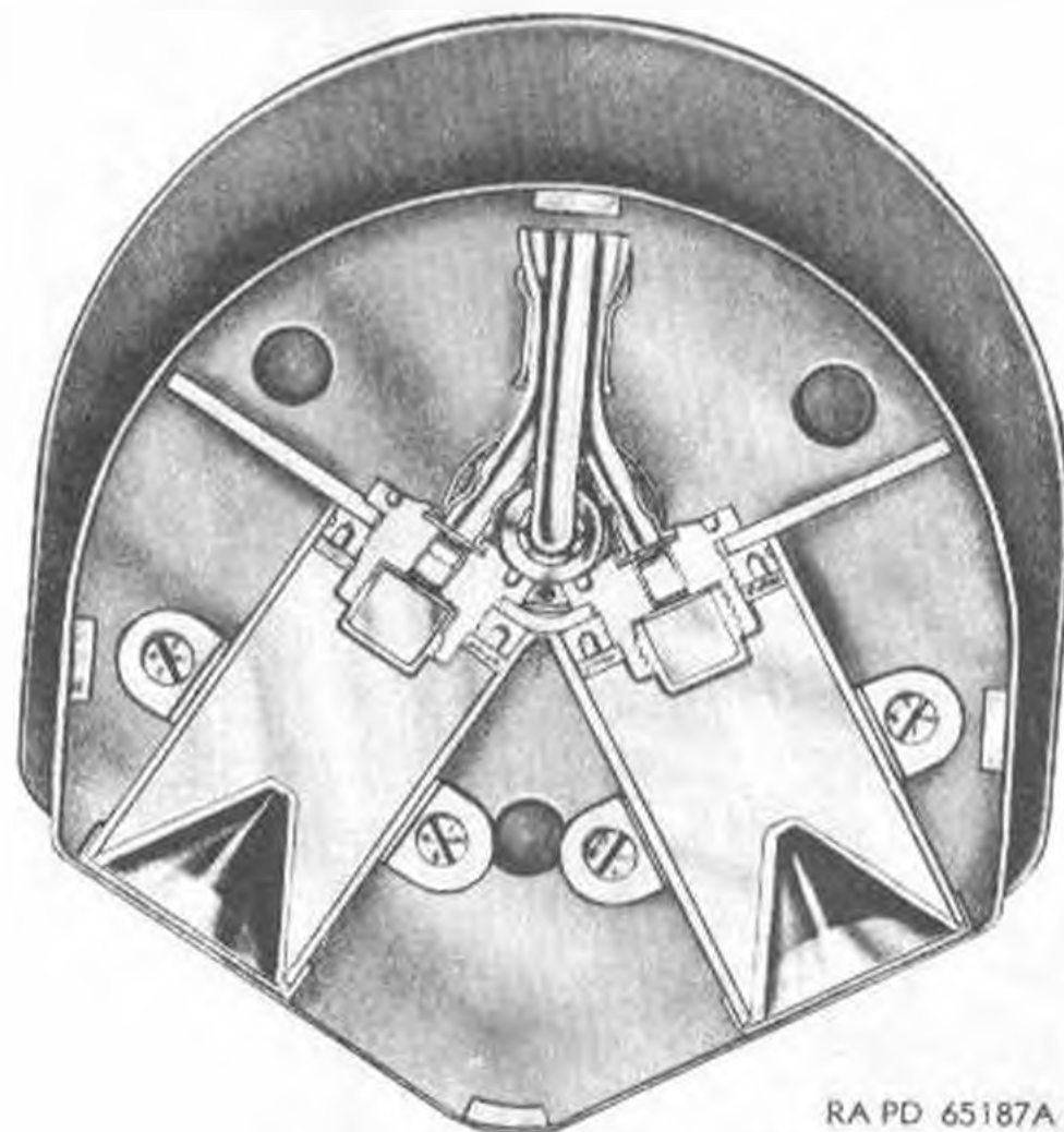
Figure 75. Fuze, bullet impact, M1A1—Cutaway and rear view.
