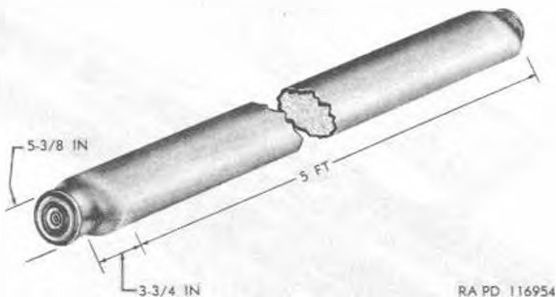
Figure 78. Charge, for snake, demolition M2A1 and M3.
