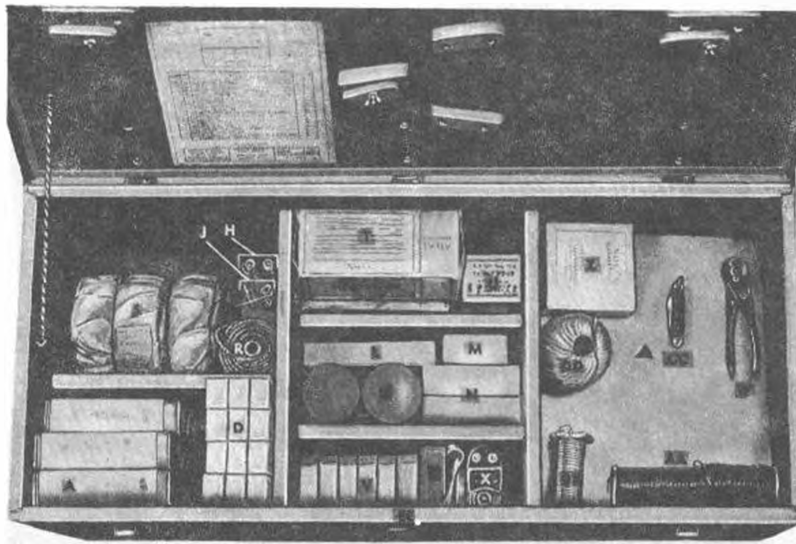
Figure 60. Demolition training kit T39—packing plan, bottom layer.
