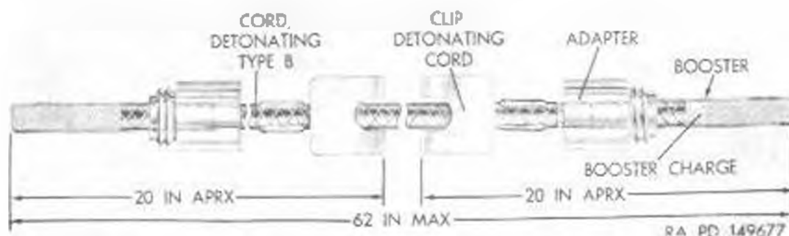
Figure 53. Priming assembly, demolition, M15.
