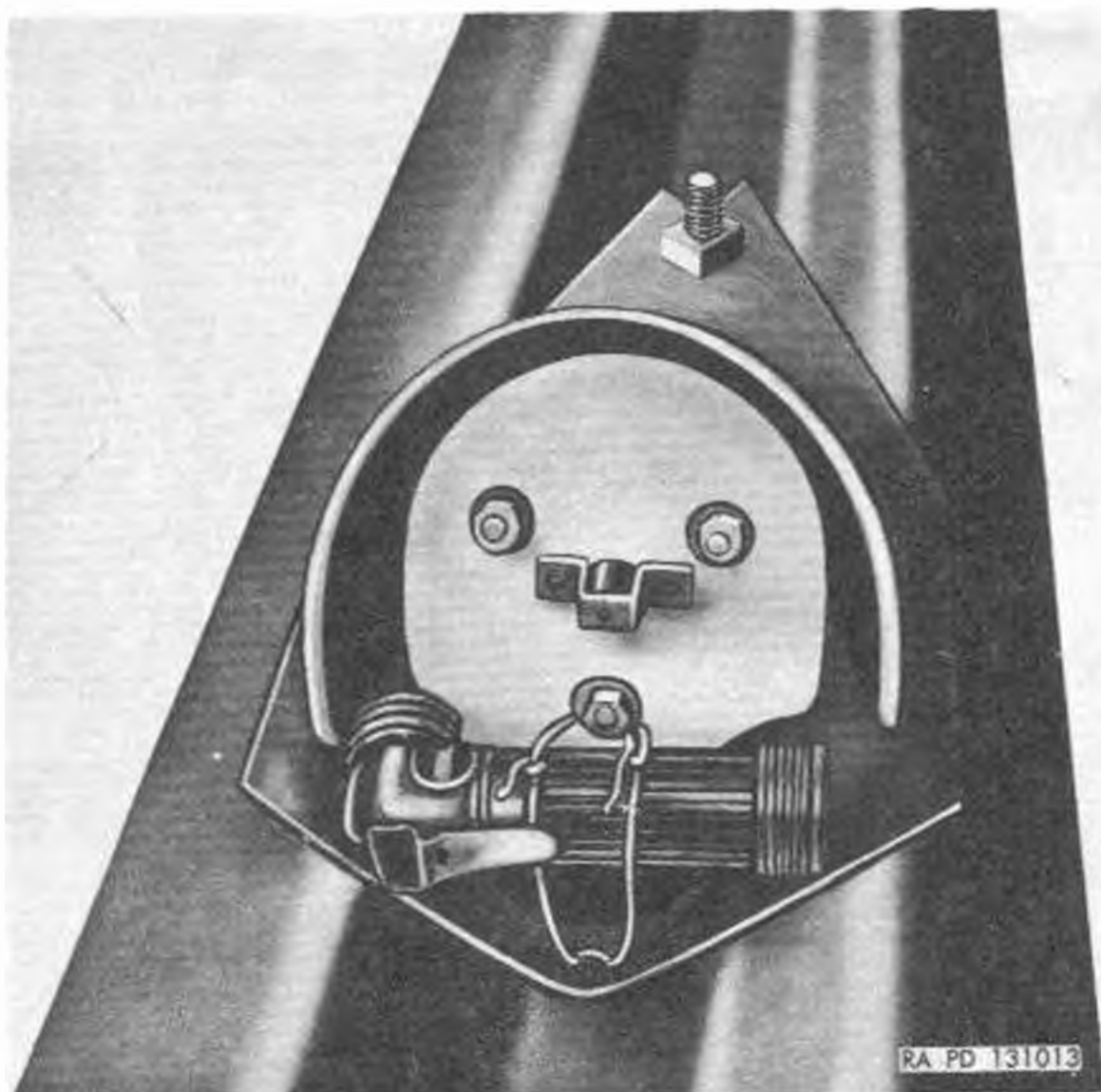
Figure 93. Fuze, bullet impact, M1, illuminated by flashlight.
