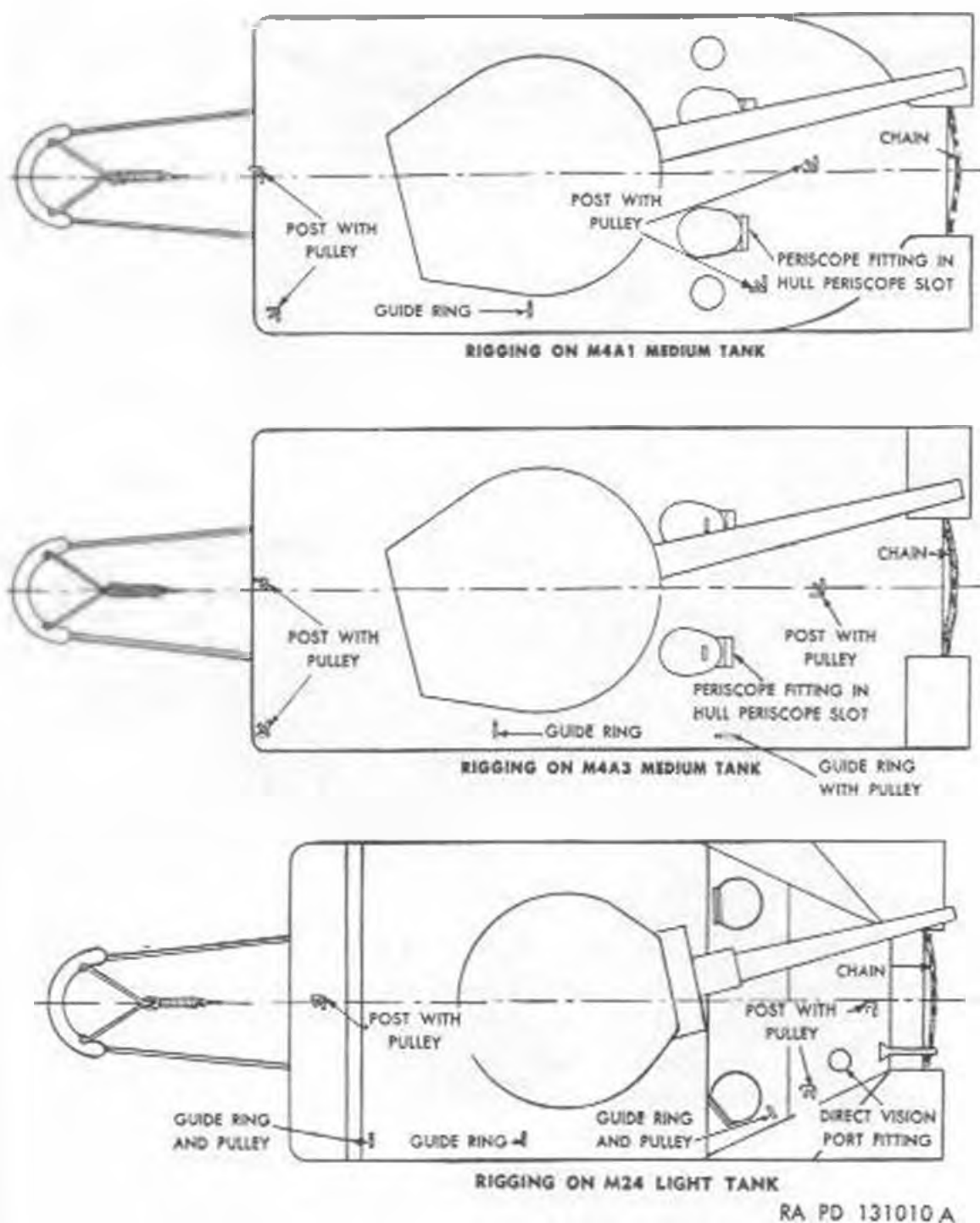
Figure 90. Location of rigging fixtures on tank hulls.
