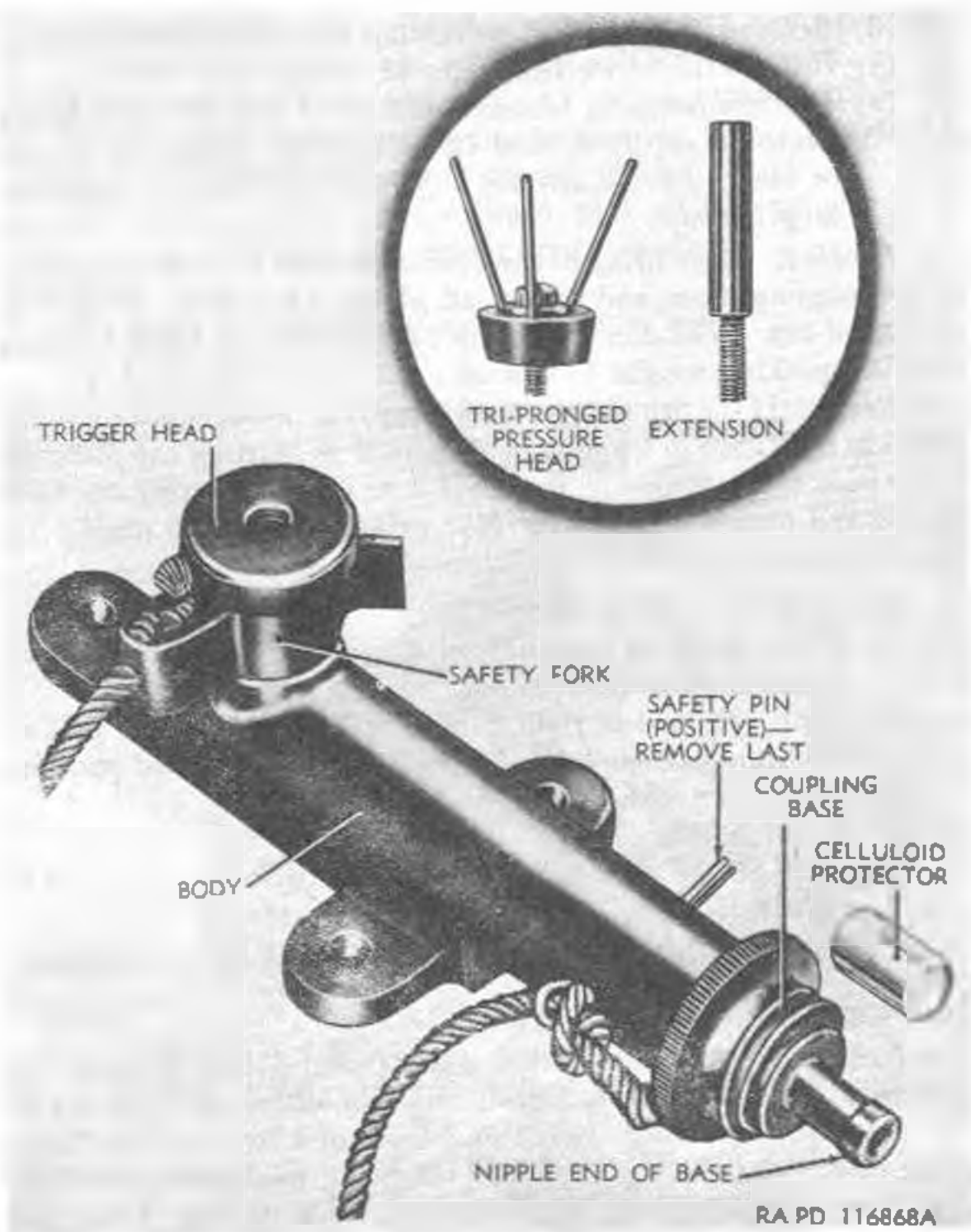
Figure 30. Firing device, pressure type, M1A1.
