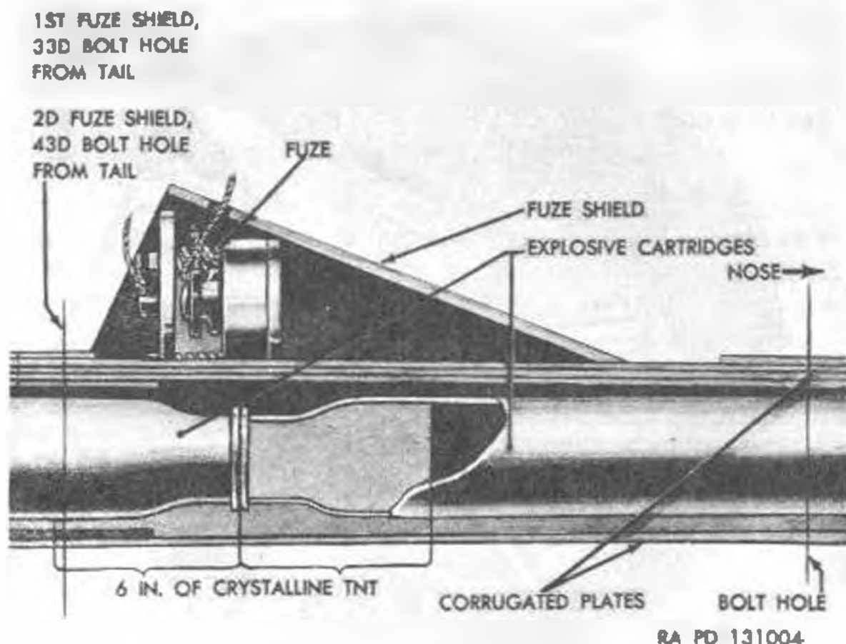
Figure 76. Longitudinal section of demolition snake M3 at fuze.
