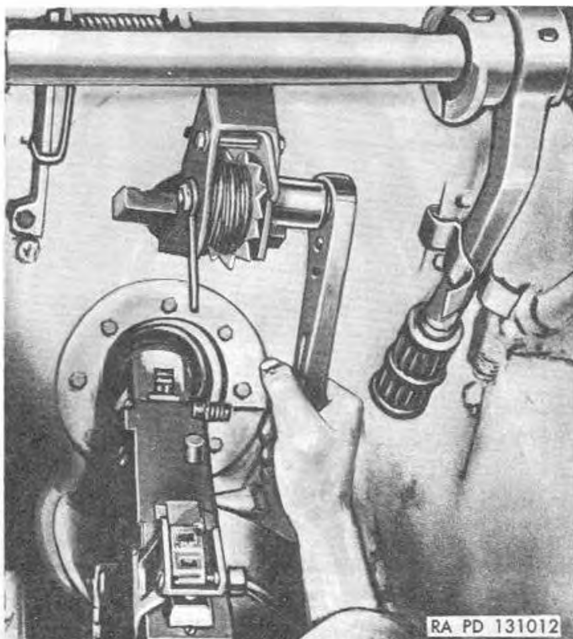
Figure 92. Light tank bow gunner raising towing assembly, using ratchet wrench.
