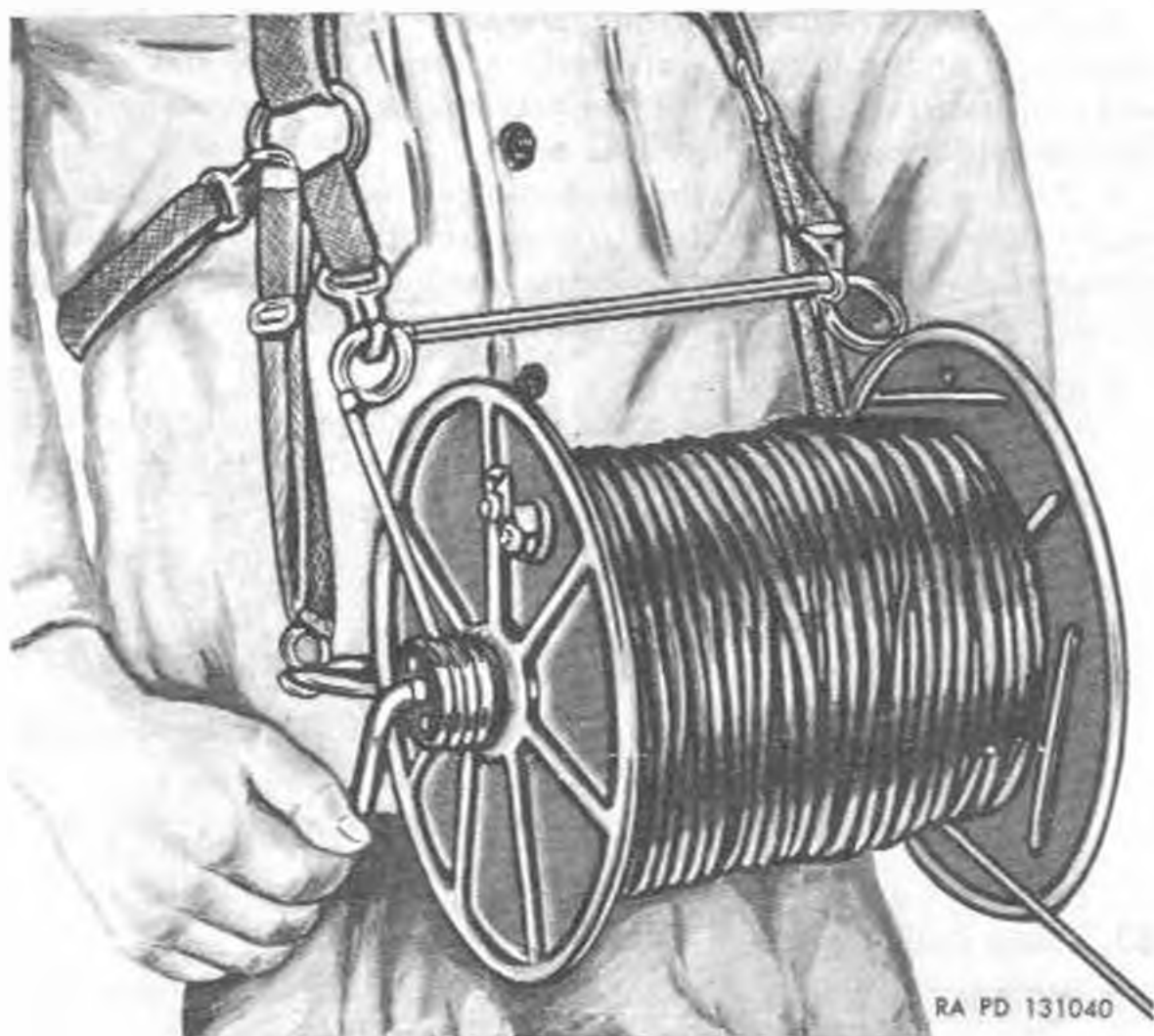
Figure 44. Reel, wire, string, 500-foot, RL-39A, with carrying straps, and wire.
