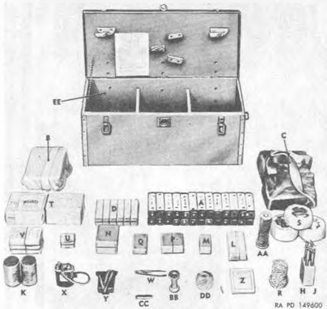
Figure 58. Demolition training kit T39.
