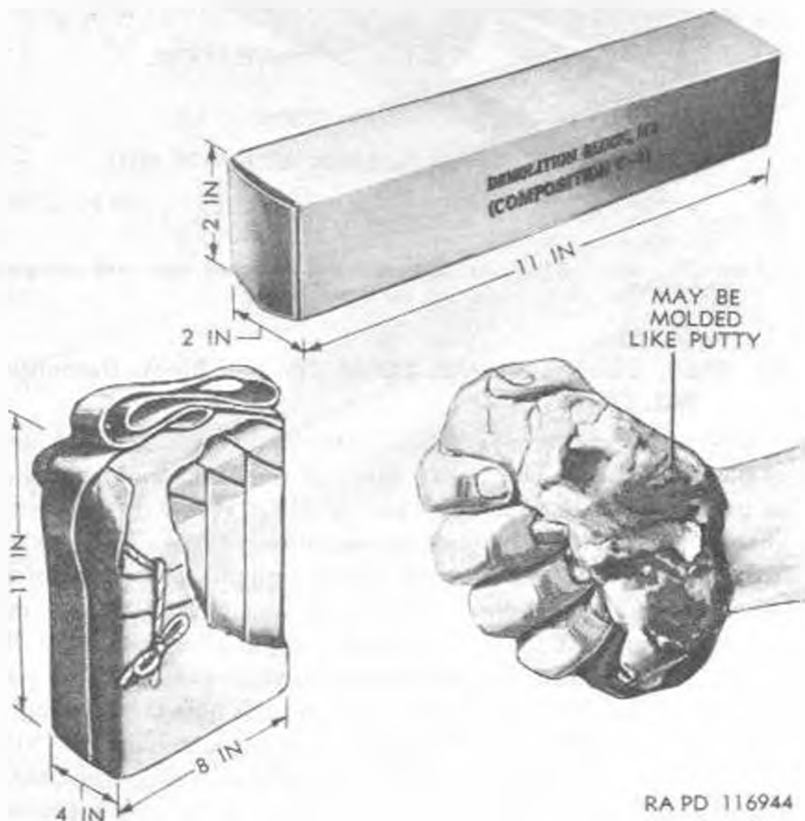
Figure 7. Block, demolition, M3 (COMP C3).
