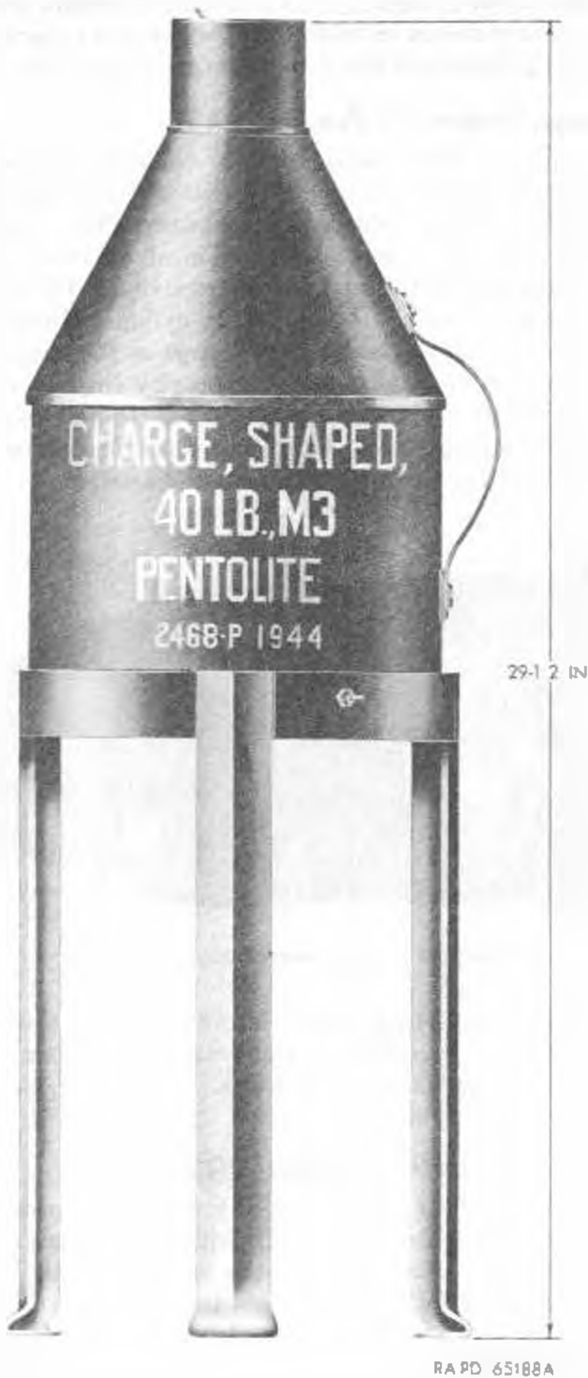
Figure 11. Charge, shaped, 40-pound, M3.
