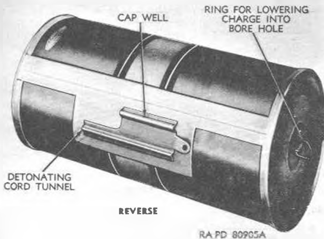
Figure 13. Charge, explosive, cratering, 40-pound, ammonium nitrate.
