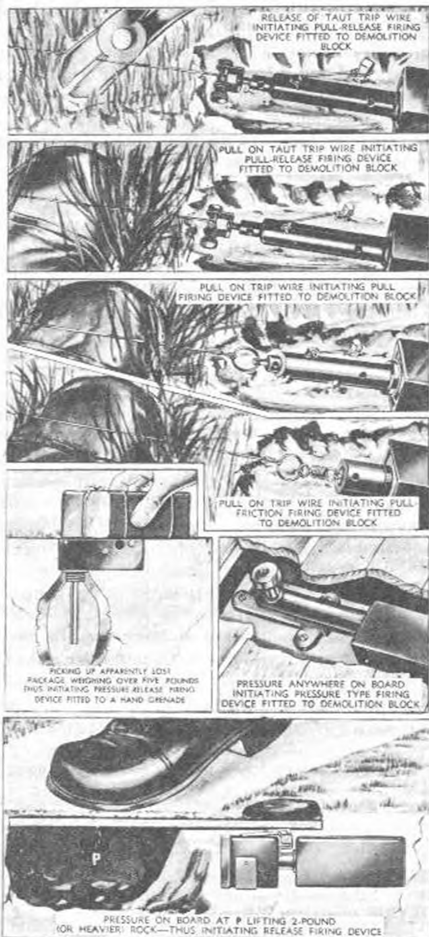
Figure 26. Representative methods of using firing devices fitted to demolition blocks for initiation by enemy troops—safety pins removed.
