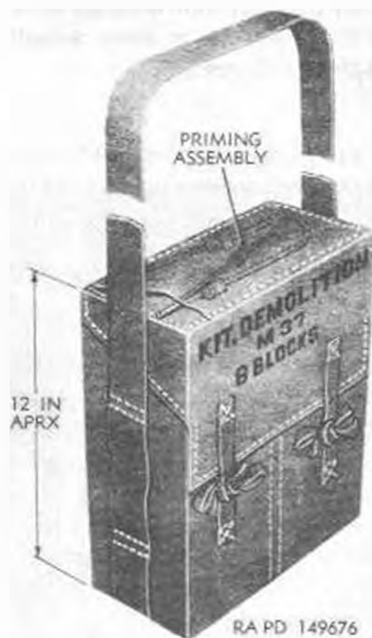
Figure 52. Kit, demolition, M37—in haversack.
