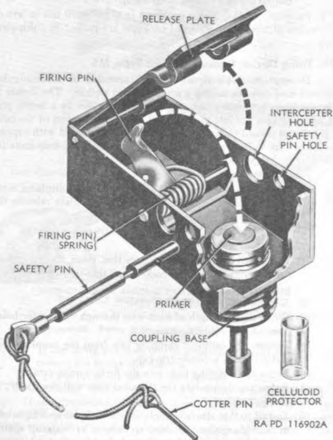
Figure 29. Firing device, pressure-release type, 315.
