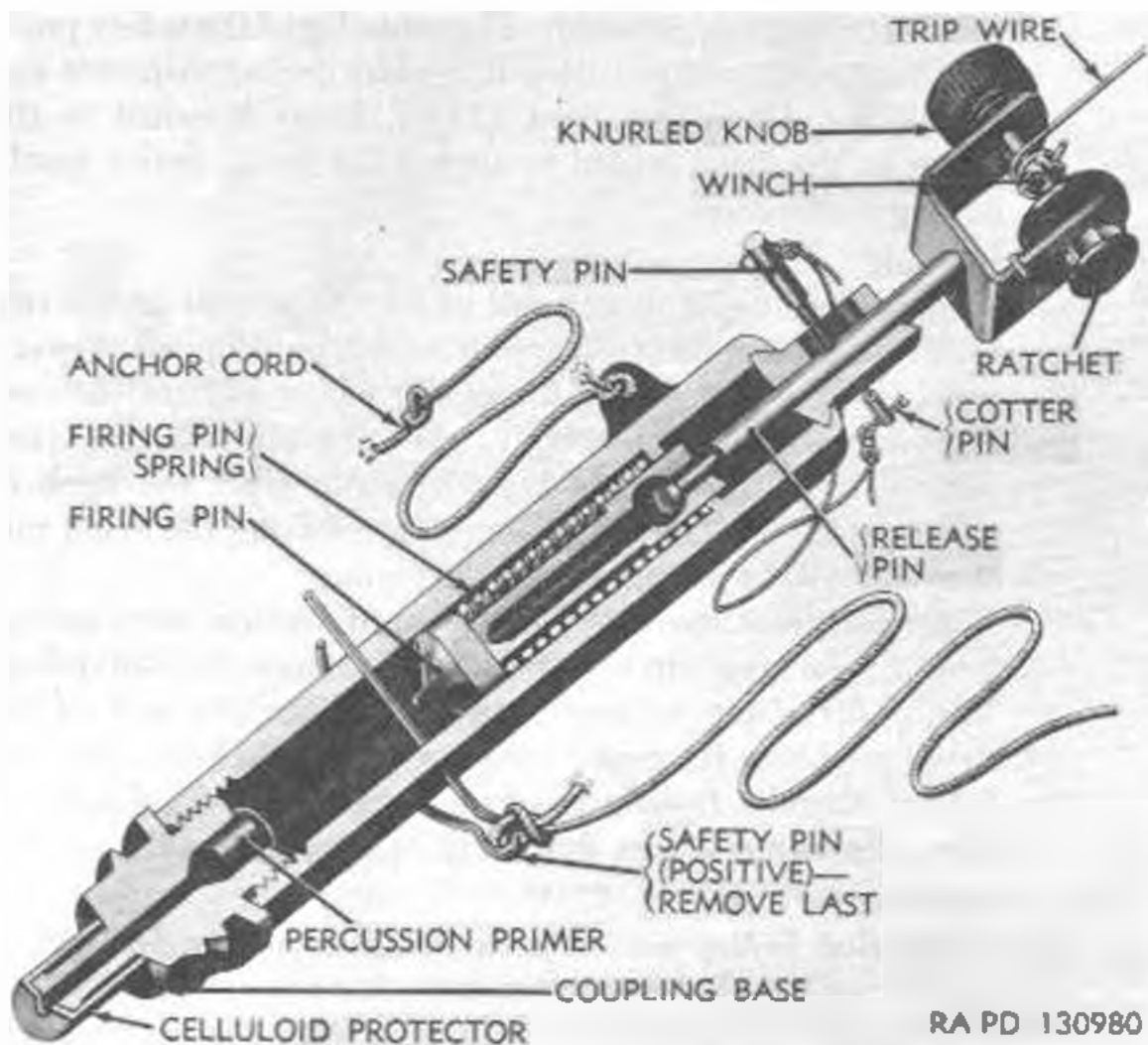
Figure 33. Firing device, pull-release type, M3—sectioned.
