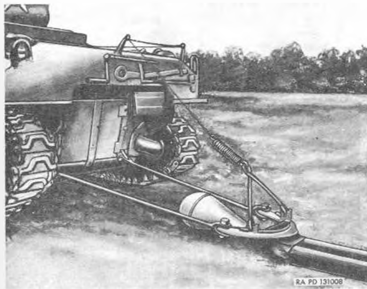
Figure 88. Towing assembly, demolition snake M3.
