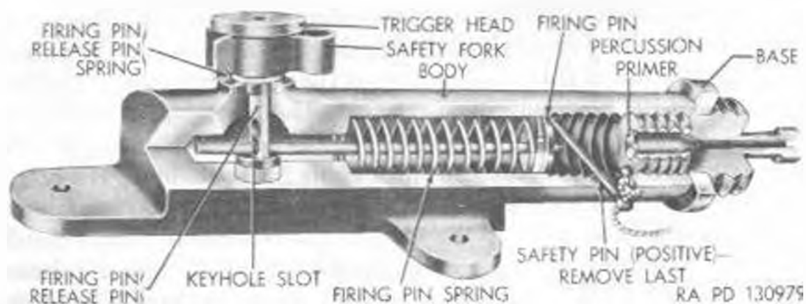
Figure 31. Firing device, pressure type, M1A1—sectioned.
