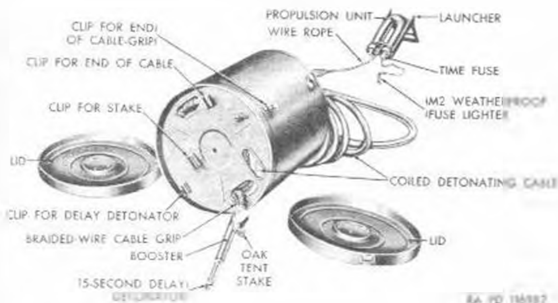
Figure 66. Cable, detonating, mine-clearing, antipersonnel, M1—ready for firing.
