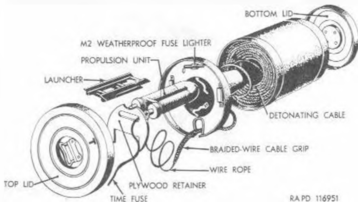
Figure 65. Cable, detonating, mine-clearing, antipersonnel, M1—arrangement of components in case.
