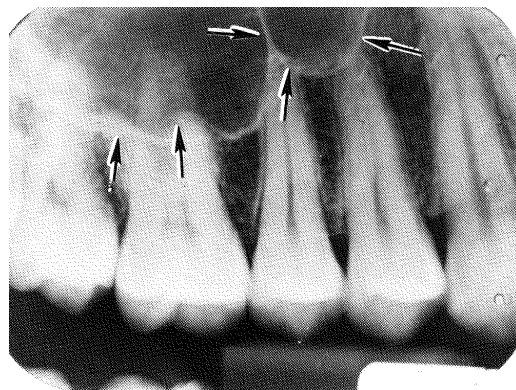
Figure 3-21. Maxillary sinus.
