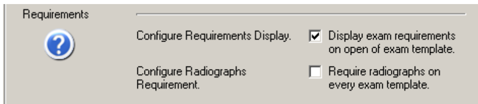
Figure 69: Requirements Parameters
