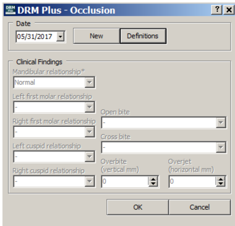
Figure 174: Occlusion Screen
