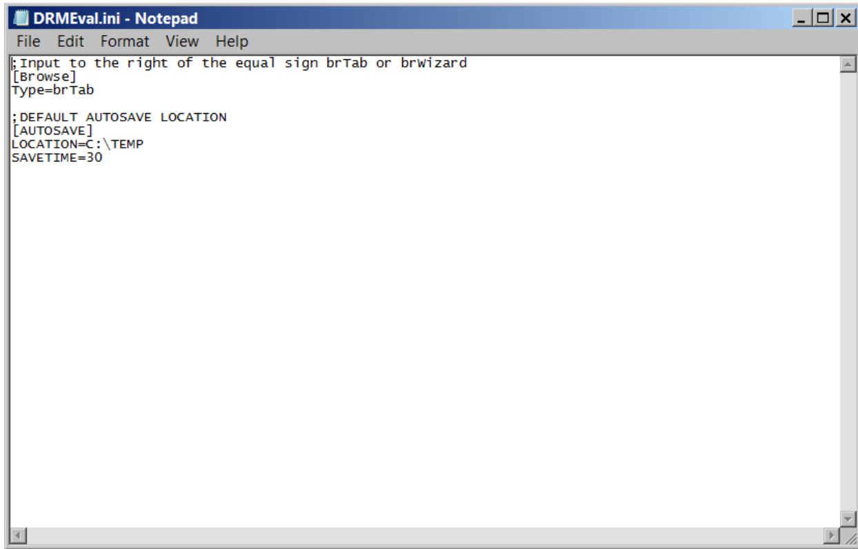
Figure 243: DRMEval.ini File
