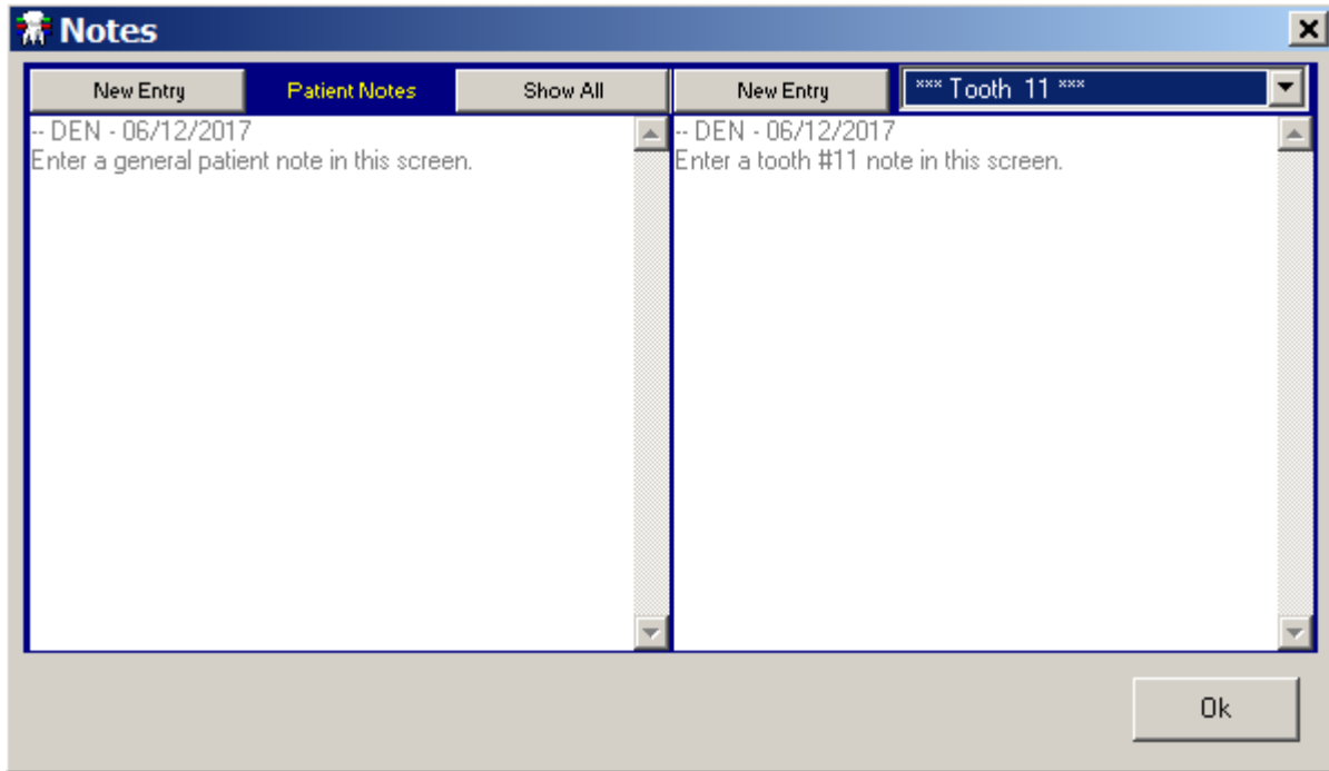
Figure 184: Notes Screen
