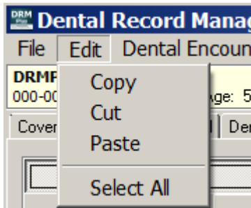
Figure 19: Edit Menu
