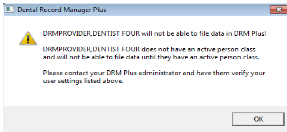
Figure 3: “!”-screen (Informational)
