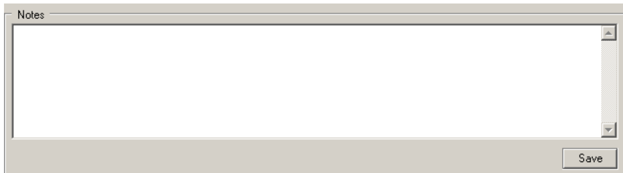
Figure 127: Notes
