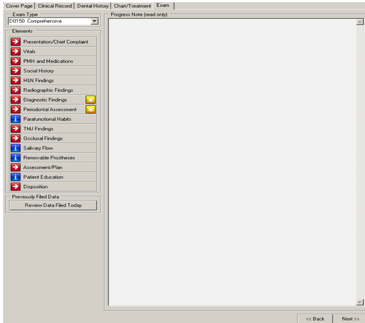
Figure 187: Exam Tab
