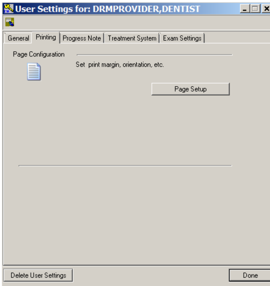
Figure 54: Printing Tab
