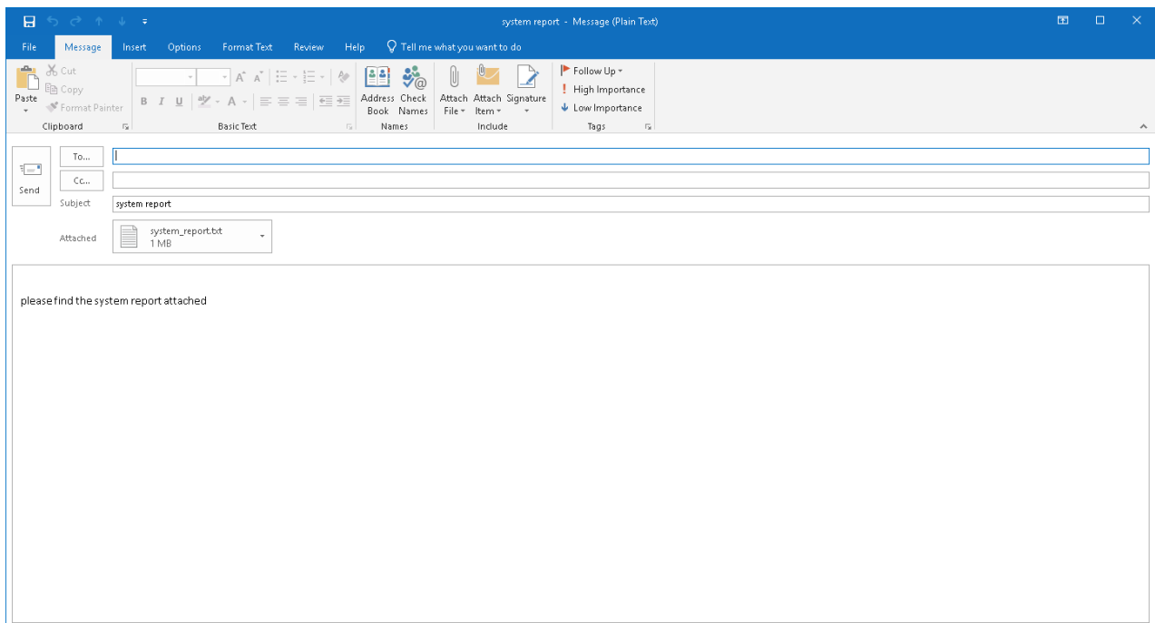
Figure 238: Outlook Window
