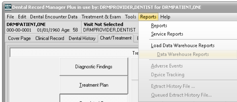
Figure 71: Reports Menu
