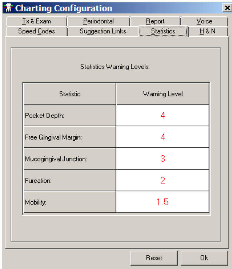
Figure 39: Statistics Tab
