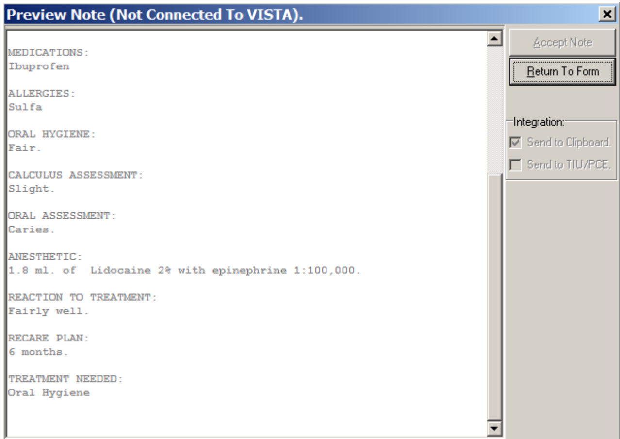
Figure 233: Preview Note
