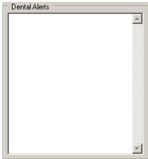
Figure 126: Dental Alerts
