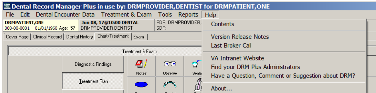
Figure 86: Help Menu
