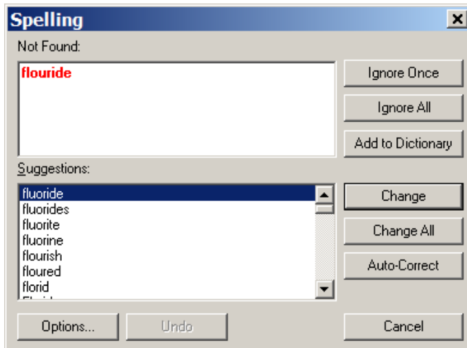
Figure 14: Spelling Screen
