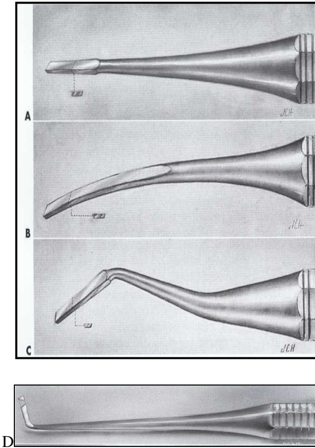
Fig . (4) Examples of hand instrument called chisels (with corresponding instrument formulas). A, Straight (12-7-0). B, Wedelstaedt (11 1 / 2 -15-3). C, Bin-angle (10-7-8) , D,Hoe.
