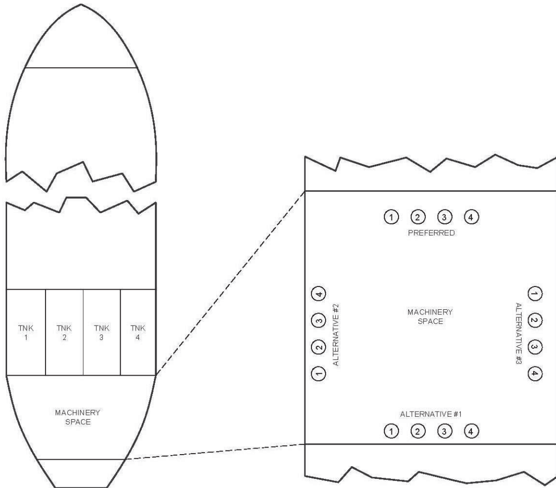
FIGURE 98. Valve manifold for tanks located athwartship.
