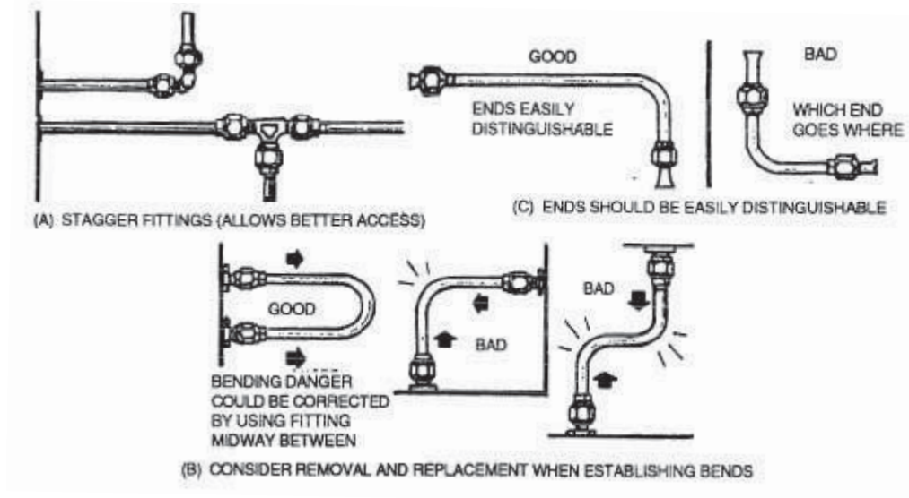
FIGURE 44. Connectors for fluid lines.
