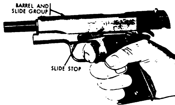
STEP 4. SLIDE GROUP LOCKED IN OPEN POSITION AFTER LAST CARTRIDGE IS FIRED.
