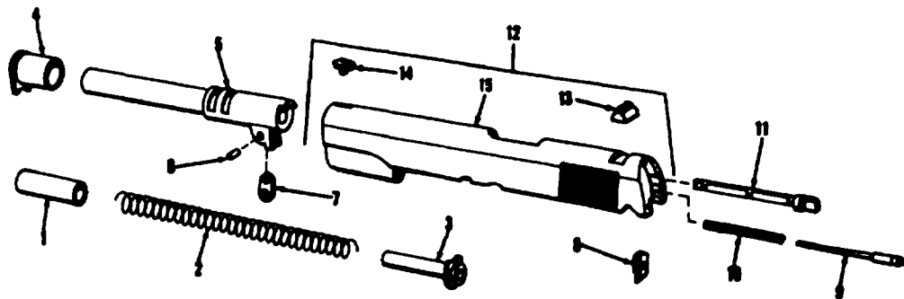
Figure B-2. Slide group.
