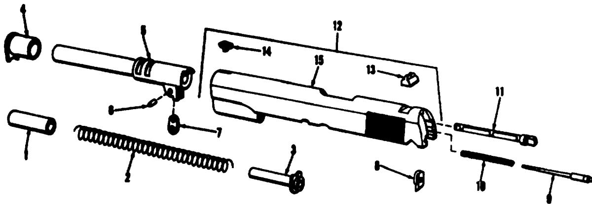
Figure B-2. Slide group-exploded view.
