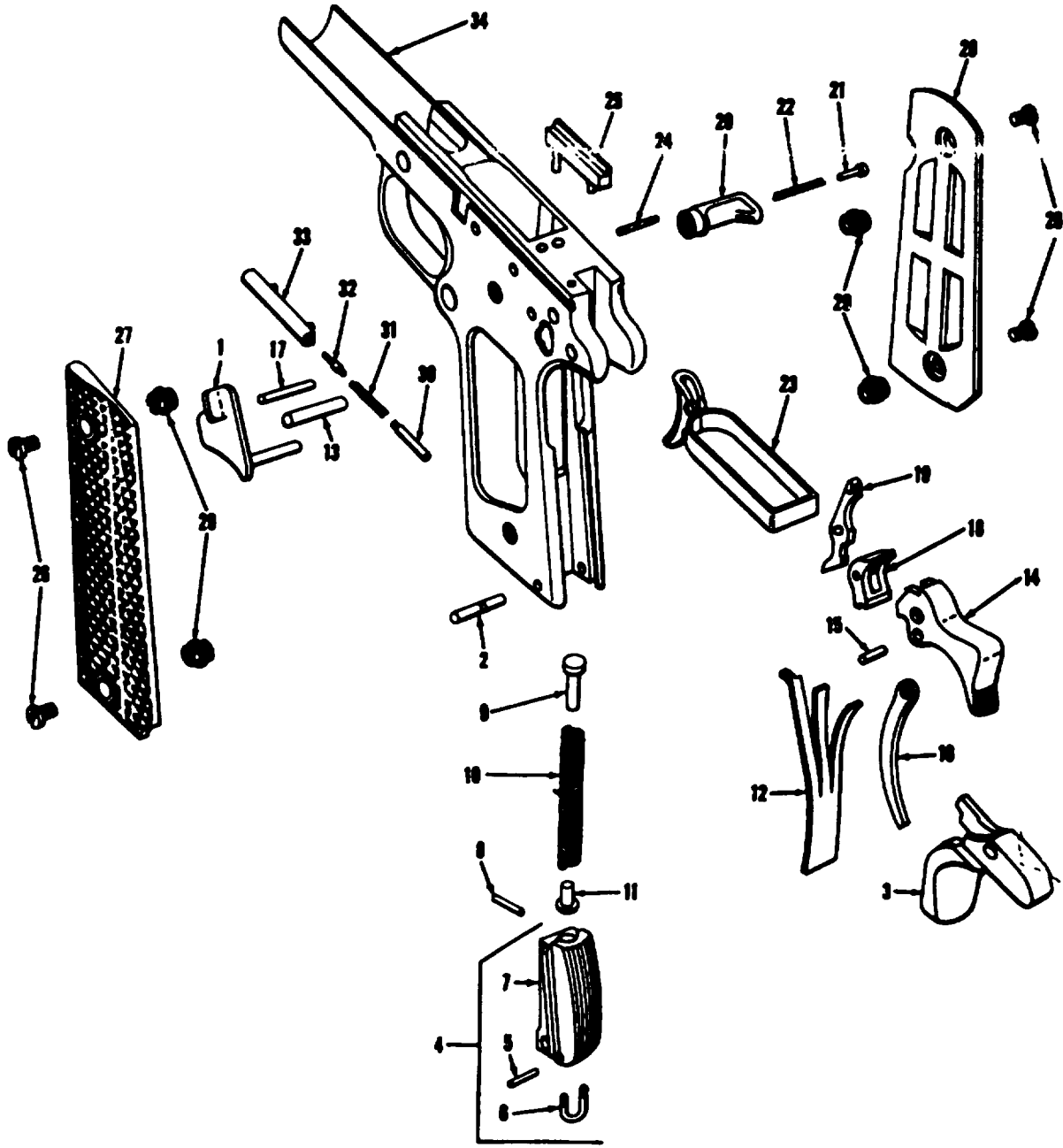
Figure B-3. Receiver group-exploded view.
