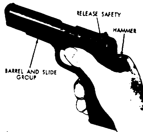
STEP 2. HAMMER COCKED - READY TO BEGIN FUNCTION FIRING.
