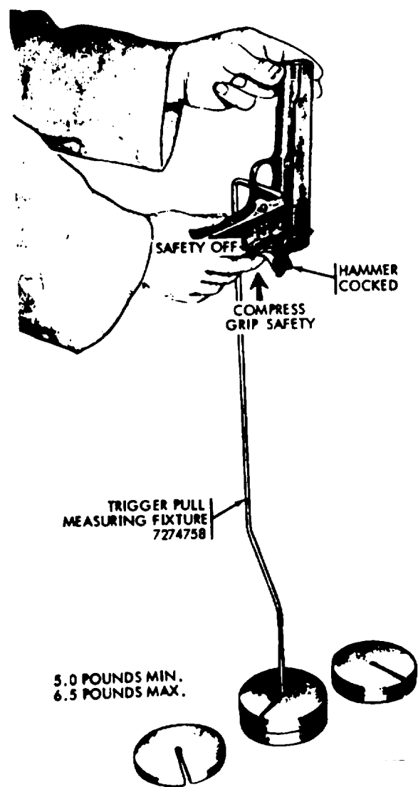
Figure 3-4. Checking trigger pull.
