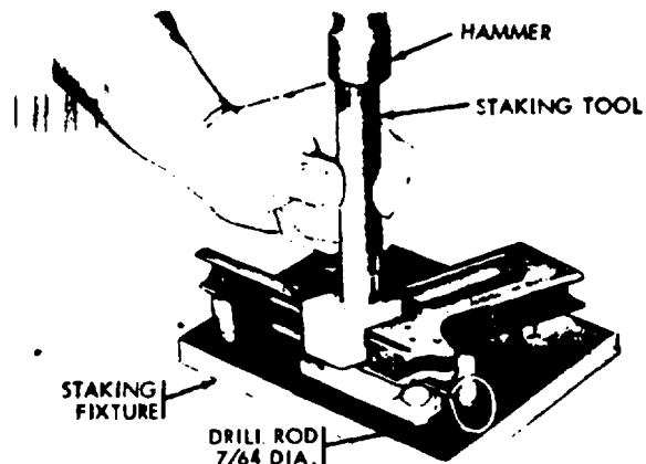
Figure 3-3. Installing and staking of plunger tube on receiver, utilizing improvised tool for staking plunger tube.
