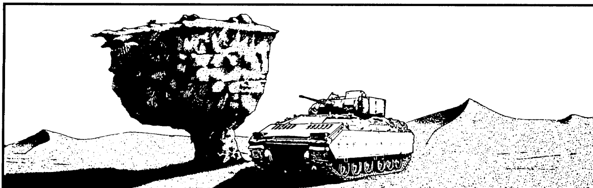
Figure 1-11. Example of wind erosion.
