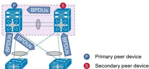
Figure 41. vPC and Spanning Tree Protocol BPDUs
