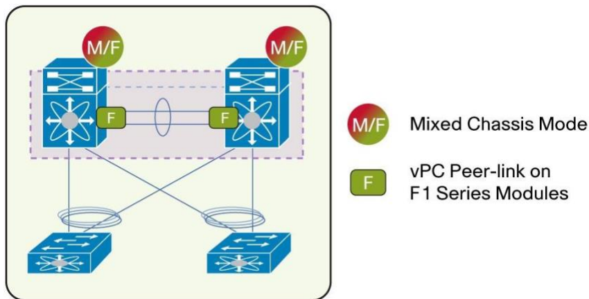
Figure 99. vPC Peer-Gateway Exclude-VLAN - Unique Topology Where the Feature Apply
