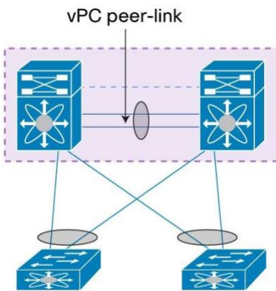
Figure 17. vPC Peer-Link
