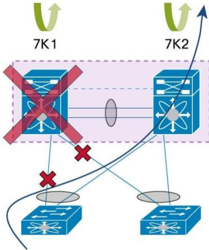
Figure 104. vPC Auto-Recovery Reload-Delay - Both vPC Peer Devices Reload But Only 7K2 Comes Back to Life
