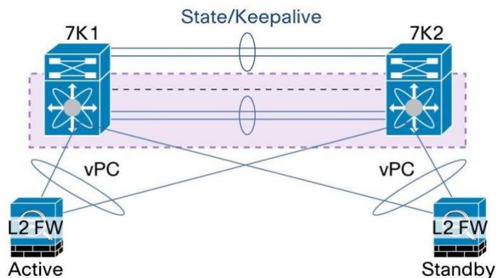
Figure 79. Network Services Appliance Configured in Transparent Mode Connected to vPC Domain
