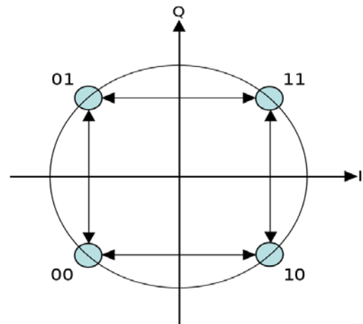
Fig5: OQPSK Constellation Diagram
