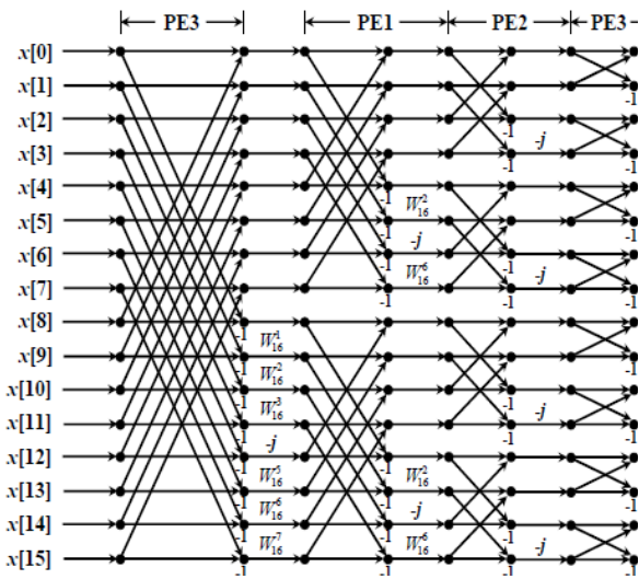
Fig. 3 Radix-2 DIF FFT signal-flow graph of length 16
