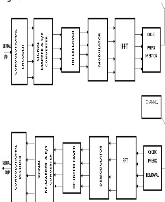
Fig. 2 OFDM Transceiver
