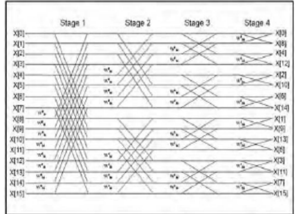
Fig. 4 Radix-2 DIT FFT signal-flow graph of length 16
