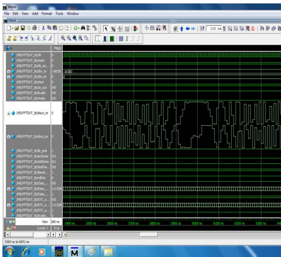
Fig 7: Output waveform of 512 point FFT processor
