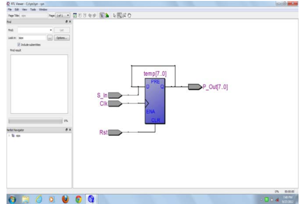
Fig 9: SIPO
