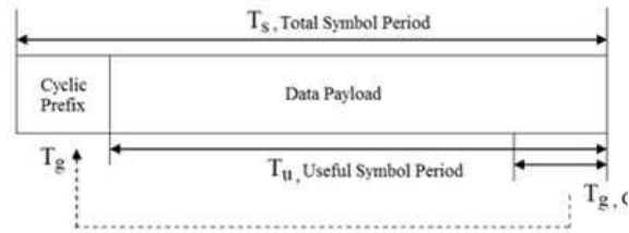
Fig6: Cycle prefix
