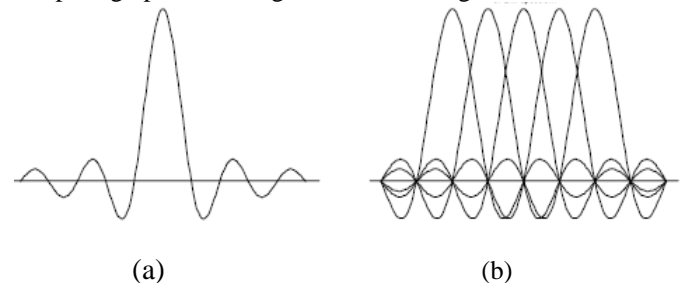
Figure 1: (a) Spectra of an OFDM sub channel and (b) an OFDM signal
