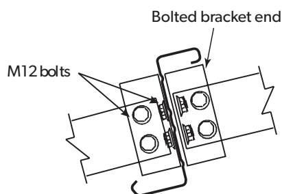
Special bridging fabricated to match the curvature of the roof
