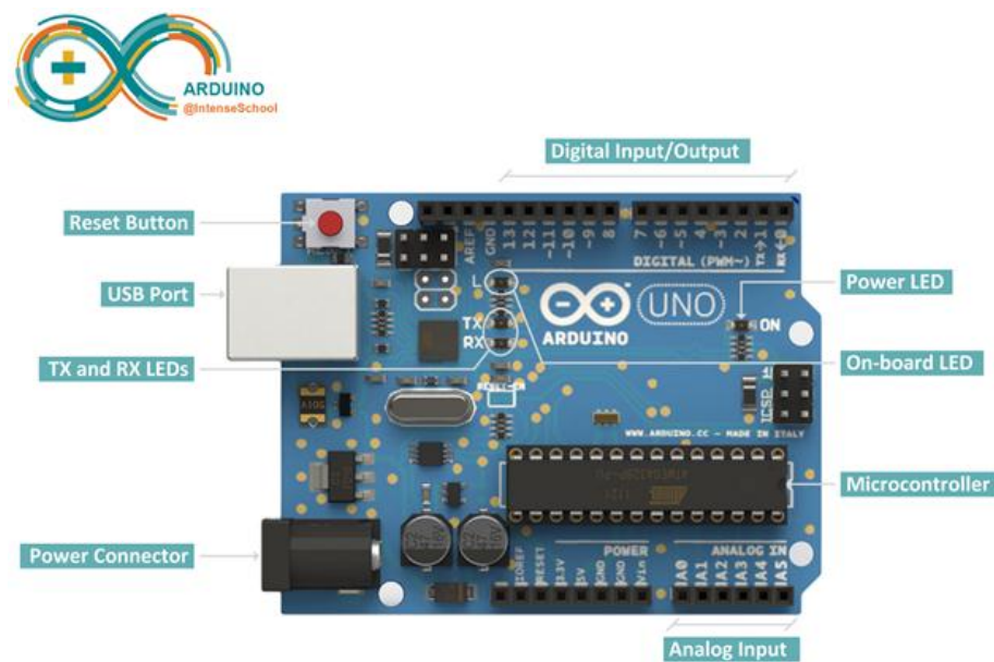
Figure3.1 Arduino Uno microcontroller board (interface)
