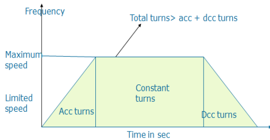
Fig. 4 : Speed profile for servo motor
