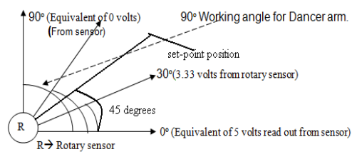
Fig. 3: Dancer arm position
