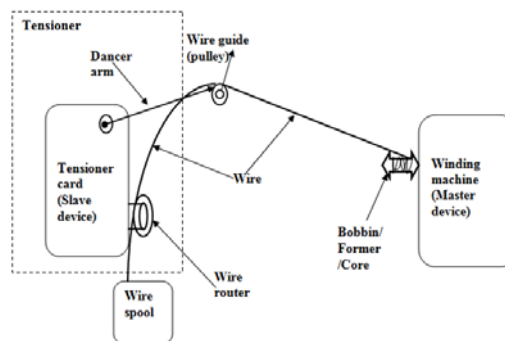
Fig. 1: Overview of Winding Machine.
