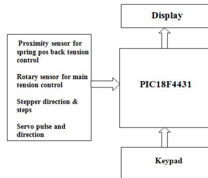
Fig. 2 : Block diagram of tensioner card
