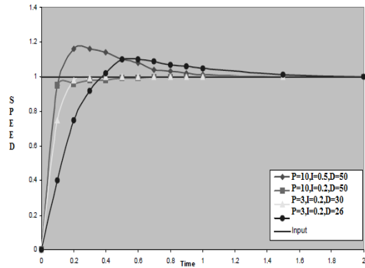
Fig. 7: PID Controller graphic Response
