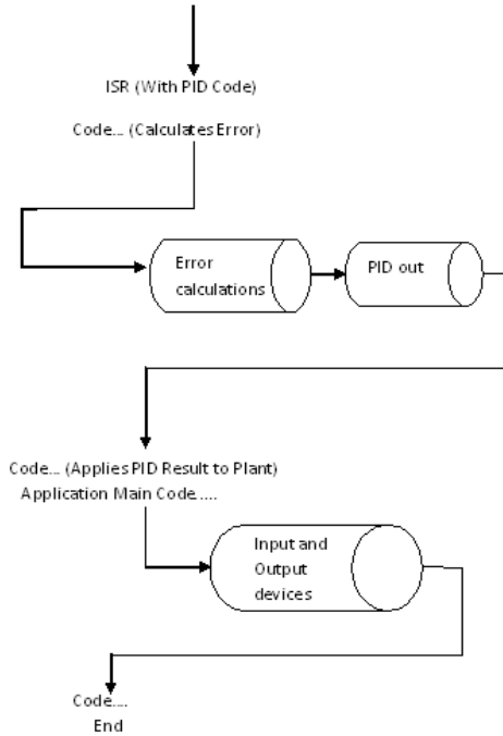
Fig. 6 : Flowchart PID firmware implementation
