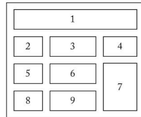
GridBagLayout
