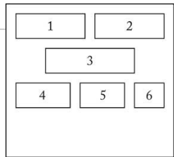
FlowLayout
