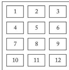
GridLayout
