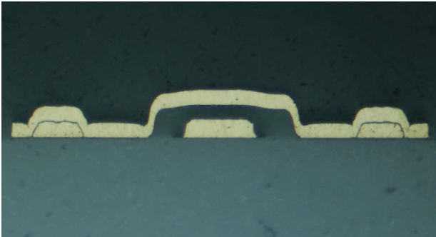
Cross-section of space-qualified polyimide-supported crossover
