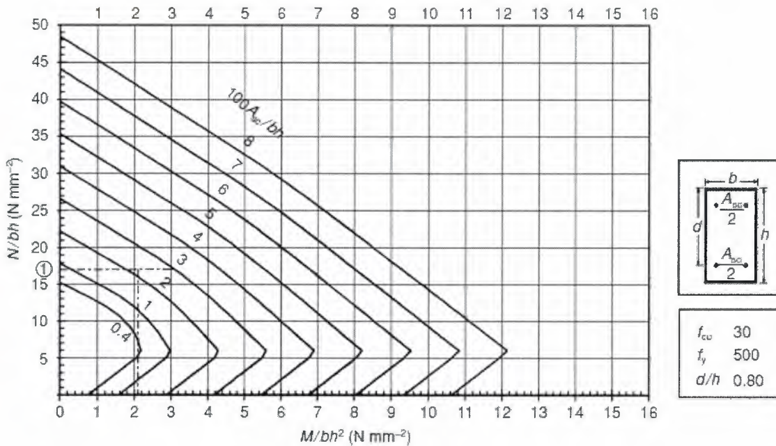
Figure 2.6: Column Design Chart (Arya, 2009)
