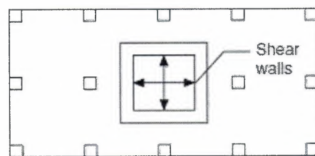
Figure 2.5: Braced Columns (Arya, 2009)
