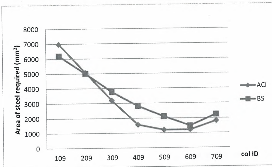
Figure 4.3: Area of Steel Required for Column 09 (Inner Column)
