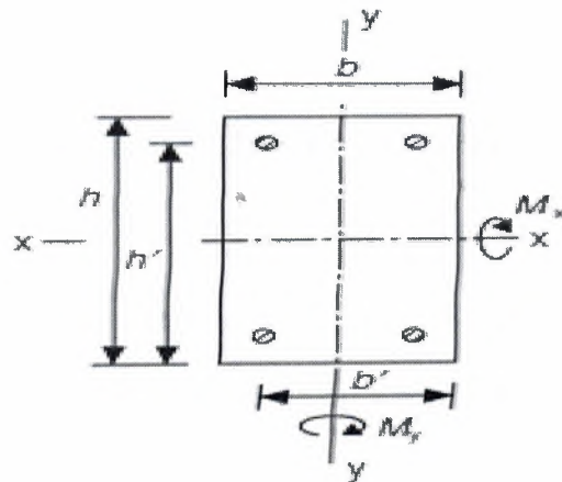
Figure 2.7: Biaxially Loaded Column (BS 8110, 1997)
