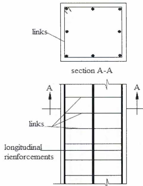
Figure 2.1: Tied Column (MacGregor, 2012)
