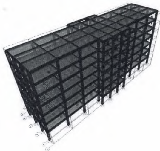
Figure 3.4: 3D Model
