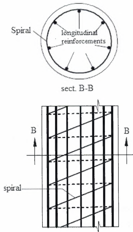
Figure 2.2: Spiral Column (MacGregor, 2012)
