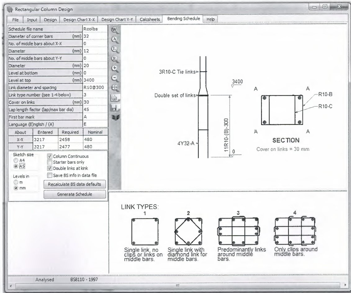
Figure 2: Prokon Bending Schedule
