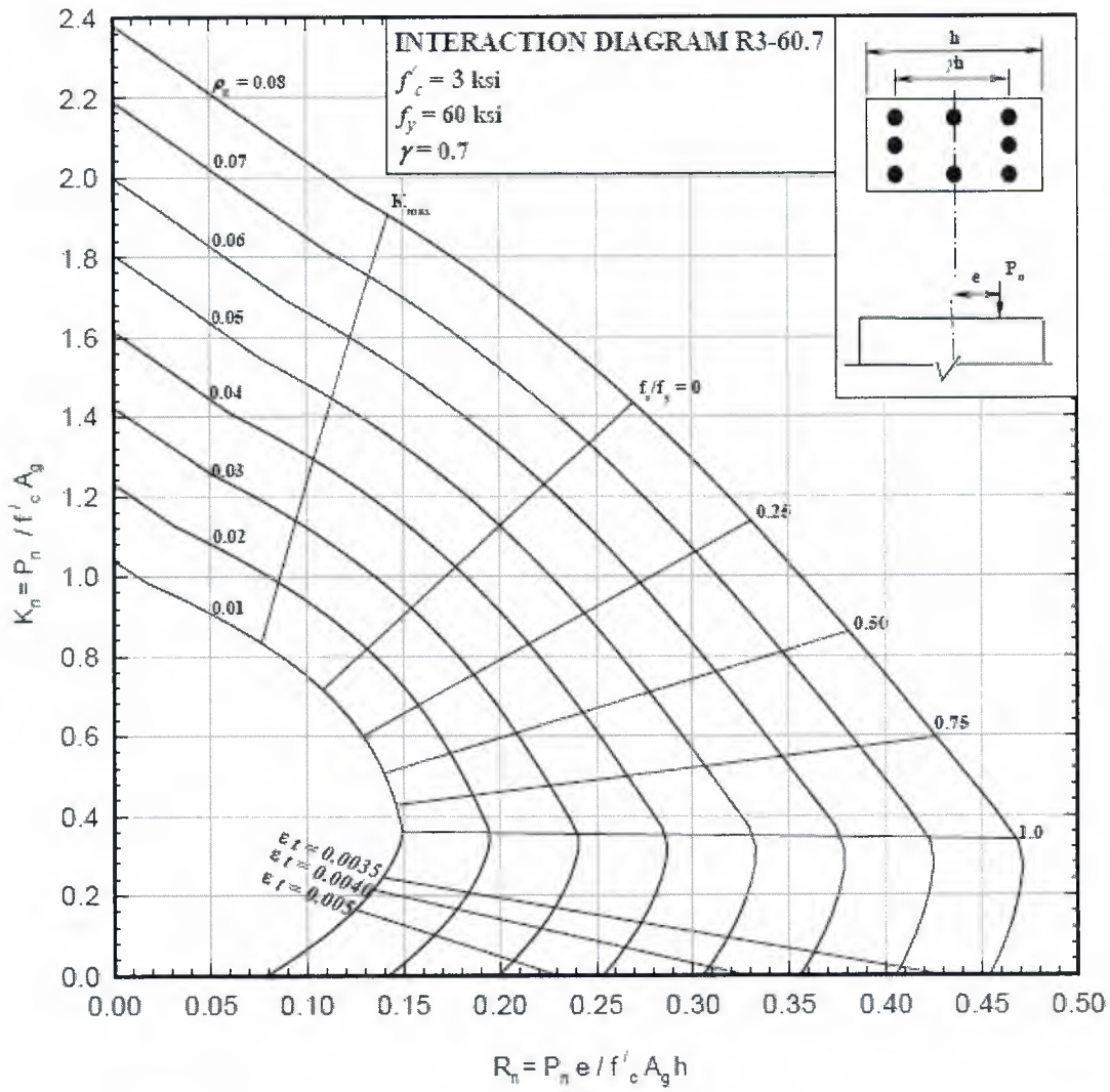
Figure 2.8: Column Interaction Diagram (Reynolds et al., 2008)
