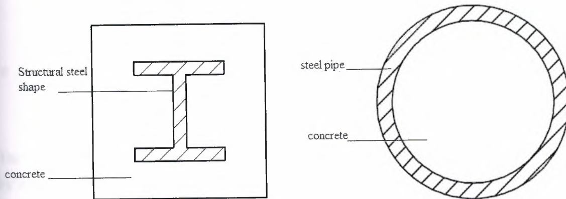
Figure 2.3: Composite Column (MacGregor, 2012)
