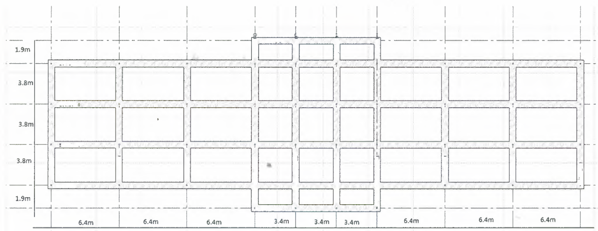
Figure 3.1: Floor plan
