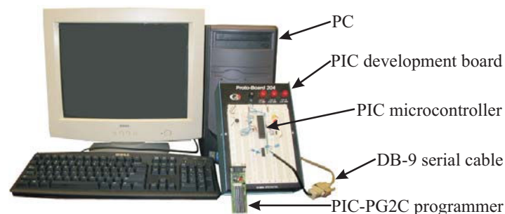
Figure 1: Hardware environment
